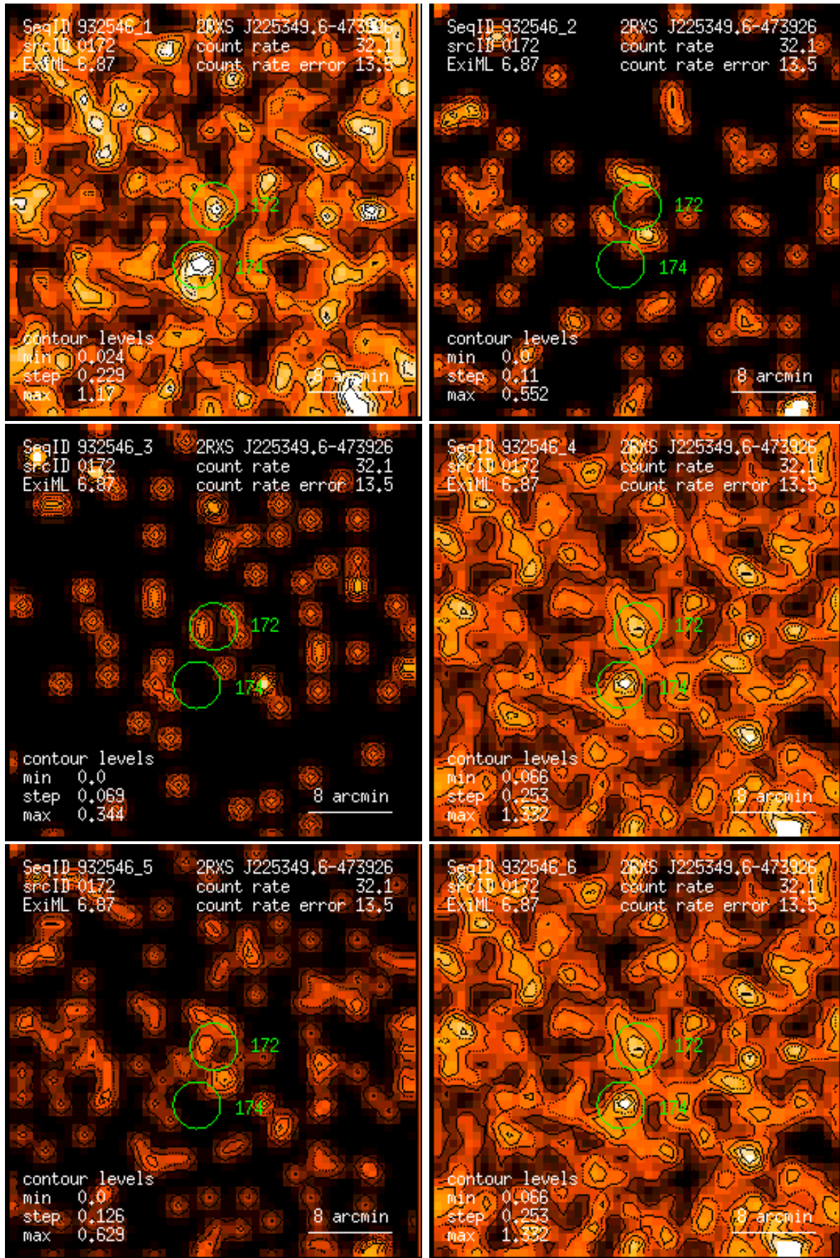
Figure 172: RASS 932546: detection 0172: band rate images, Gaussian filter: (1) PSPC channels 11 – 41, (2) 52 – 90, (3) 91 – 201, (4) 11 – 235, (5) 52 – 201, (6) 11 – 201. Broad band rates in counts/ks. Band rate contour levels in counts/ks/arcmin 2 .
