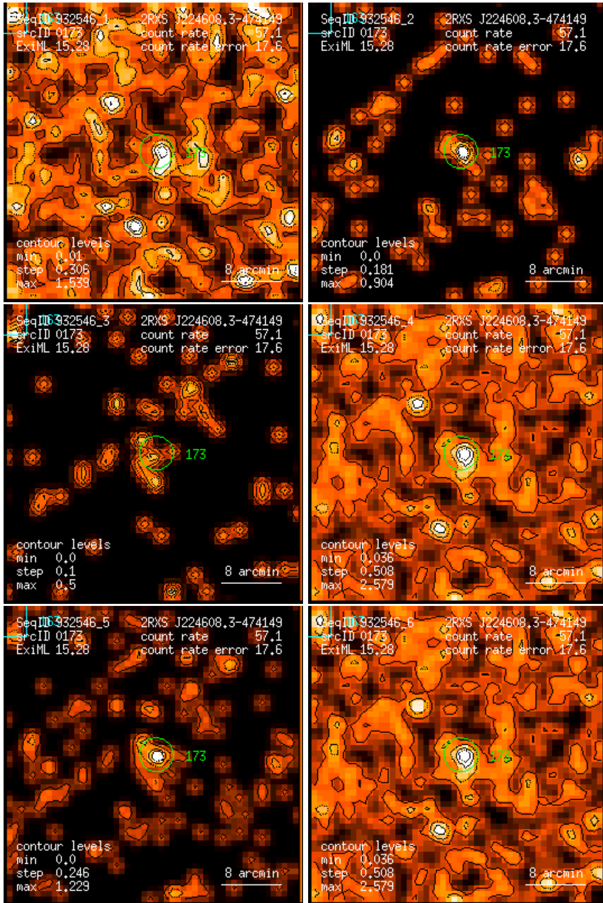
Figure 173: RASS 932546: detection 0173: band rate images, Gaussian filter: (1) PSPC channels 11 – 41, (2) 52 – 90, (3) 91 – 201, (4) 11 – 235, (5) 52 – 201, (6) 11 – 201. Broad band rates in counts/ks. Band rate contour levels in counts/ks/arcmin 2 .
