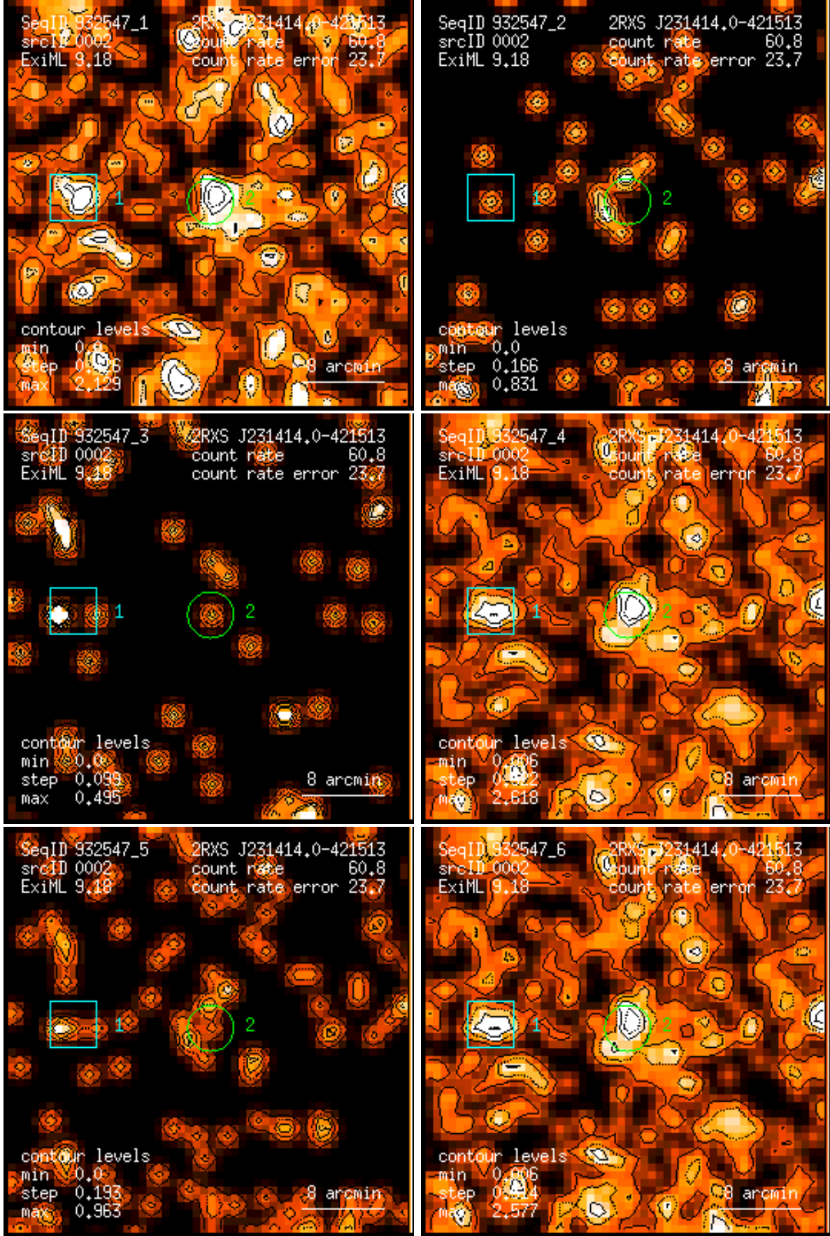
Figure 2: RASS 932547: detection 0002: band rate images, Gaussian filter: (1) PSPC channels 11 – 41, (2) 52 – 90, (3) 91 – 201, (4) 11 – 235, (5) 52 – 201, (6) 11 – 201. Broad band rates in counts/ks. Band rate contour levels in counts/ks/arcmin 2 .
