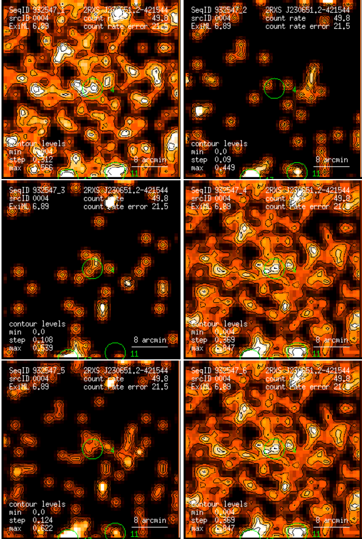
Figure 4: RASS 932547: detection 0004: band rate images, Gaussian filter: (1) PSPC channels 11 – 41, (2) 52 – 90, (3) 91 – 201, (4) 11 – 235, (5) 52 – 201, (6) 11 – 201. Broad band rates in counts/ks. Band rate contour levels in counts/ks/arcmin 2 .
