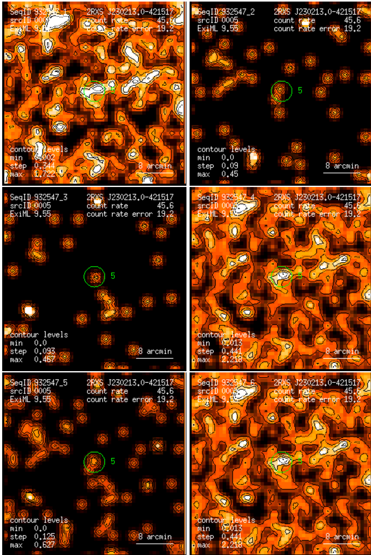
Figure 5: RASS 932547: detection 0005: band rate images, Gaussian filter: (1) PSPC channels 11 – 41, (2) 52 – 90, (3) 91 – 201, (4) 11 – 235, (5) 52 – 201, (6) 11 – 201. Broad band rates in counts/ks. Band rate contour levels in counts/ks/arcmin 2 .
