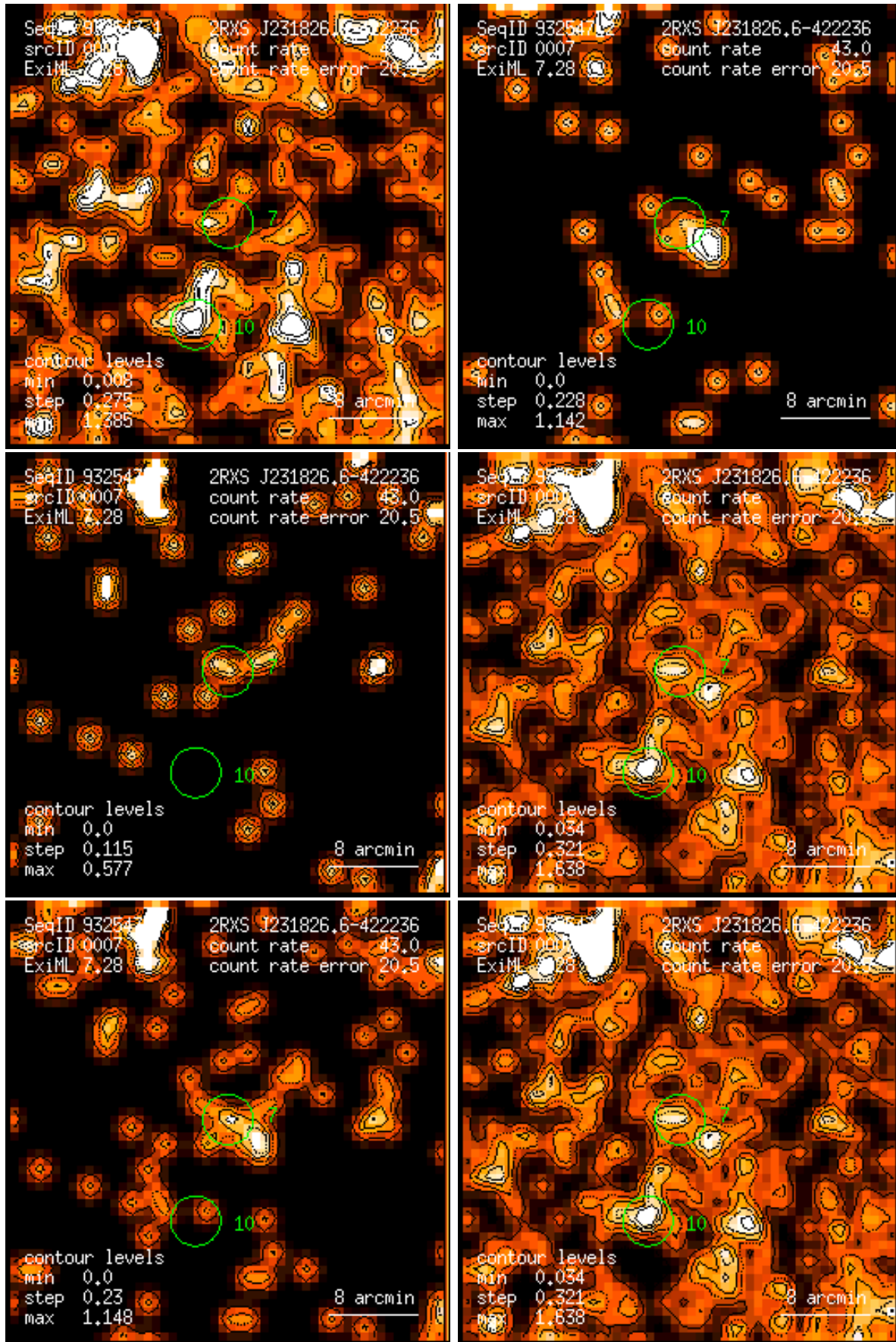
Figure 7: RASS 932547: detection 0007: band rate images, Gaussian filter: (1) PSPC channels 11 – 41, (2) 52 – 90, (3) 91 – 201, (4) 11 – 235, (5) 52 – 201, (6) 11 – 201. Broad band rates in counts/ks. Band rate contour levels in counts/ks/arcmin 2 .
