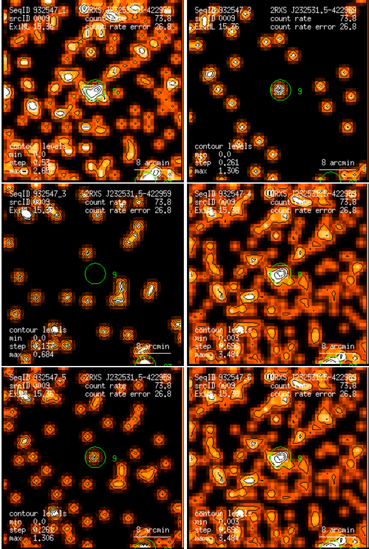
Figure 9: RASS 932547: detection 0009: band rate images, Gaussian filter: (1) PSPC channels 11 – 41, (2) 52 – 90, (3) 91 – 201, (4) 11 – 235, (5) 52 – 201, (6) 11 – 201. Broad band rates in counts/ks. Band rate contour levels in counts/ks/arcmin 2 .
