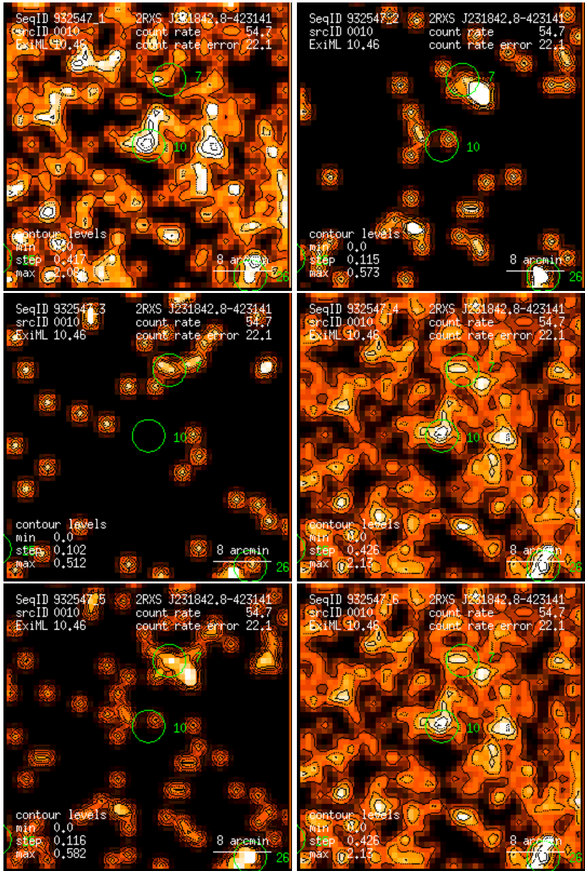
Figure 10: RASS 932547: detection 0010: band rate images, Gaussian filter: (1) PSPC channels 11 – 41, (2) 52 – 90, (3) 91 – 201, (4) 11 – 235, (5) 52 – 201, (6) 11 – 201. Broad band rates in counts/ks. Band rate contour levels in counts/ks/arcmin 2 .
