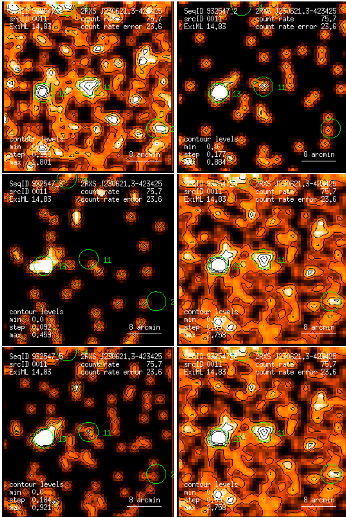
Figure 11: RASS 932547: detection 0011: band rate images, Gaussian filter: (1) PSPC channels 11 – 41, (2) 52 – 90, (3) 91 – 201, (4) 11 – 235, (5) 52 – 201, (6) 11 – 201. Broad band rates in counts/ks. Band rate contour levels in counts/ks/arcmin 2 .
