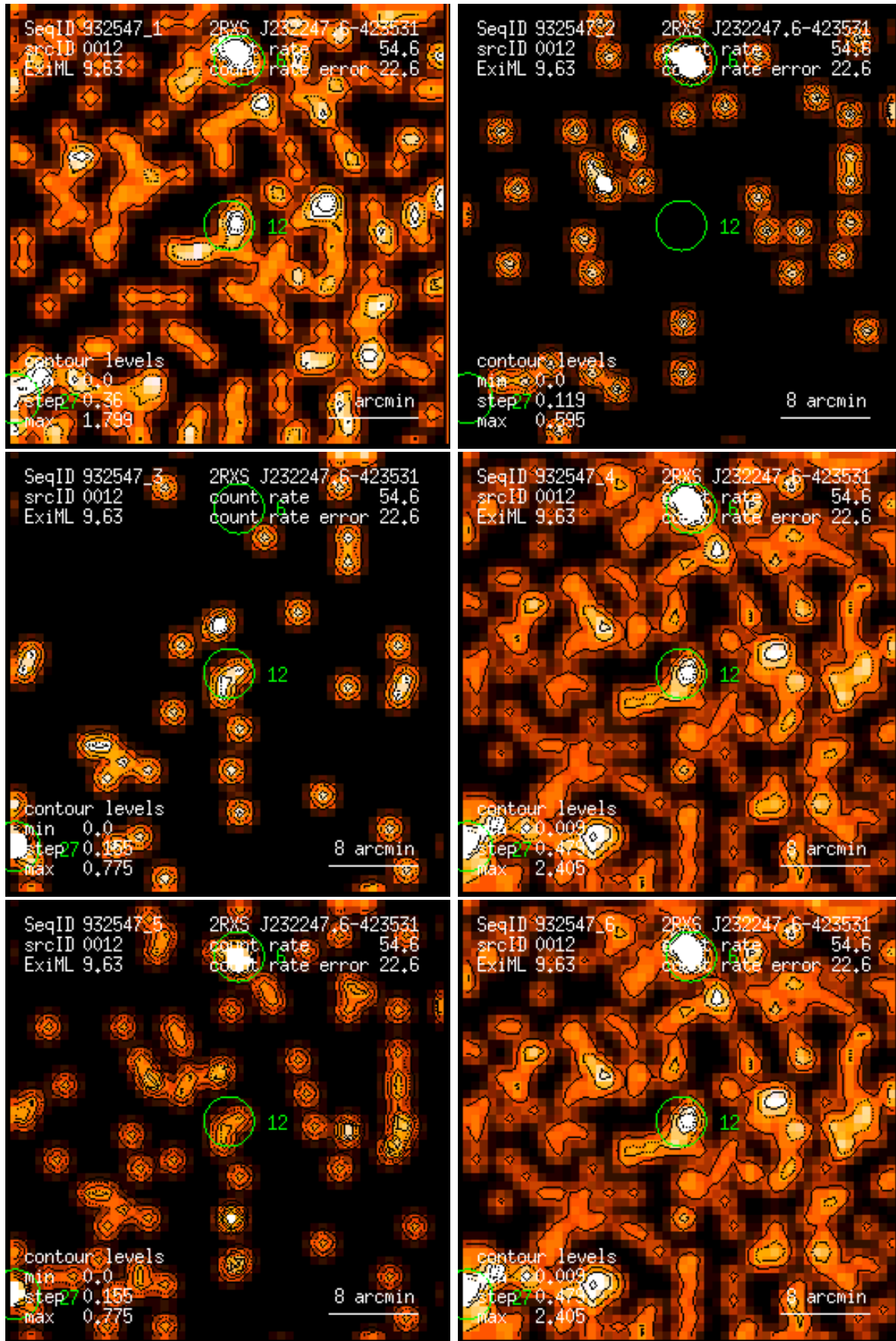
Figure 12: RASS 932547: detection 0012: band rate images, Gaussian filter: (1) PSPC channels 11 – 41, (2) 52 – 90, (3) 91 – 201, (4) 11 – 235, (5) 52 – 201, (6) 11 – 201. Broad band rates in counts/ks. Band rate contour levels in counts/ks/arcmin 2 .
