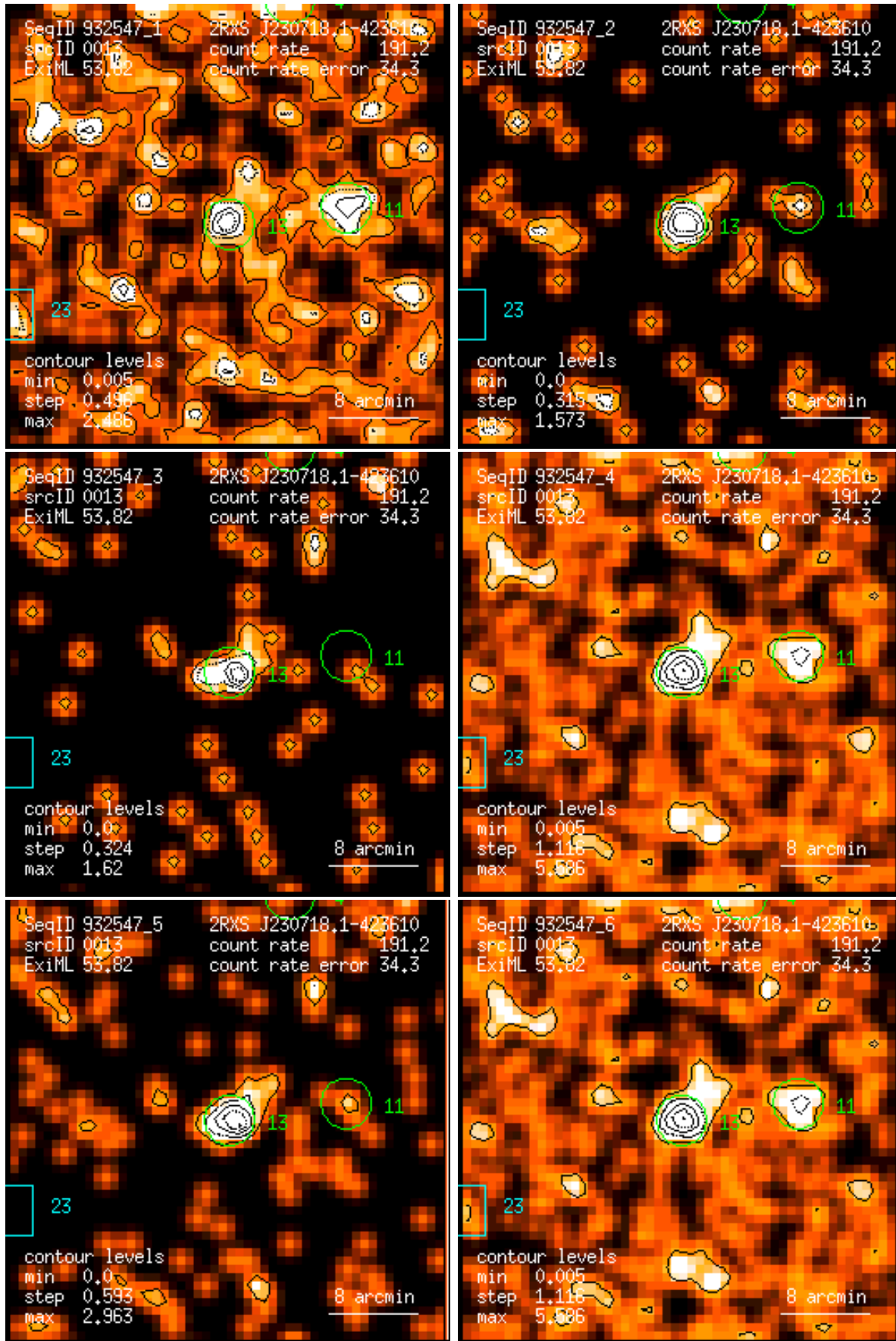
Figure 13: RASS 932547: detection 0013: band rate images, Gaussian filter: (1) PSPC channels 11 – 41, (2) 52 – 90, (3) 91 – 201, (4) 11 – 235, (5) 52 – 201, (6) 11 – 201. Broad band rates in counts/ks. Band rate contour levels in counts/ks/arcmin 2 .
