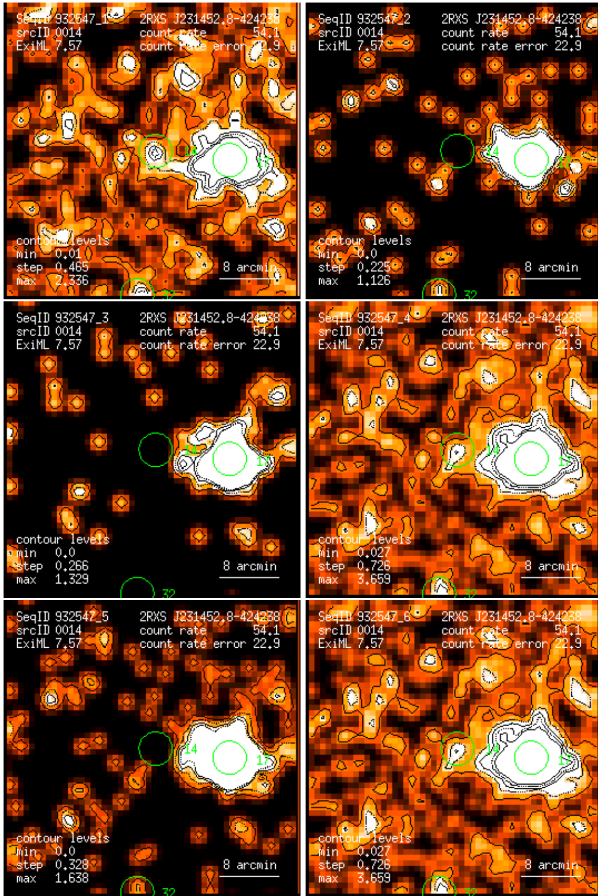
Figure 14: RASS 932547: detection 0014: band rate images, Gaussian filter: (1) PSPC channels 11 – 41, (2) 52 – 90, (3) 91 – 201, (4) 11 – 235, (5) 52 – 201, (6) 11 – 201. Broad band rates in counts/ks. Band rate contour levels in counts/ks/arcmin 2 .
