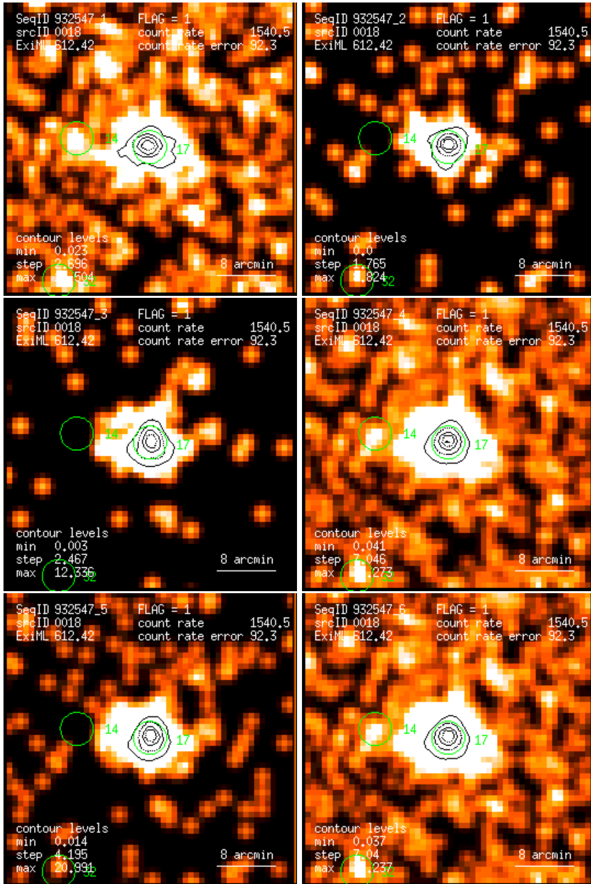
Figure 18: RASS 932547: detection 0018: band rate images, Gaussian filter: (1) PSPC channels 11 – 41, (2) 52 – 90, (3) 91 – 201, (4) 11 – 235, (5) 52 – 201, (6) 11 – 201. Broad band rates in counts/ks. Band rate contour levels in counts/ks/arcmin 2 .
