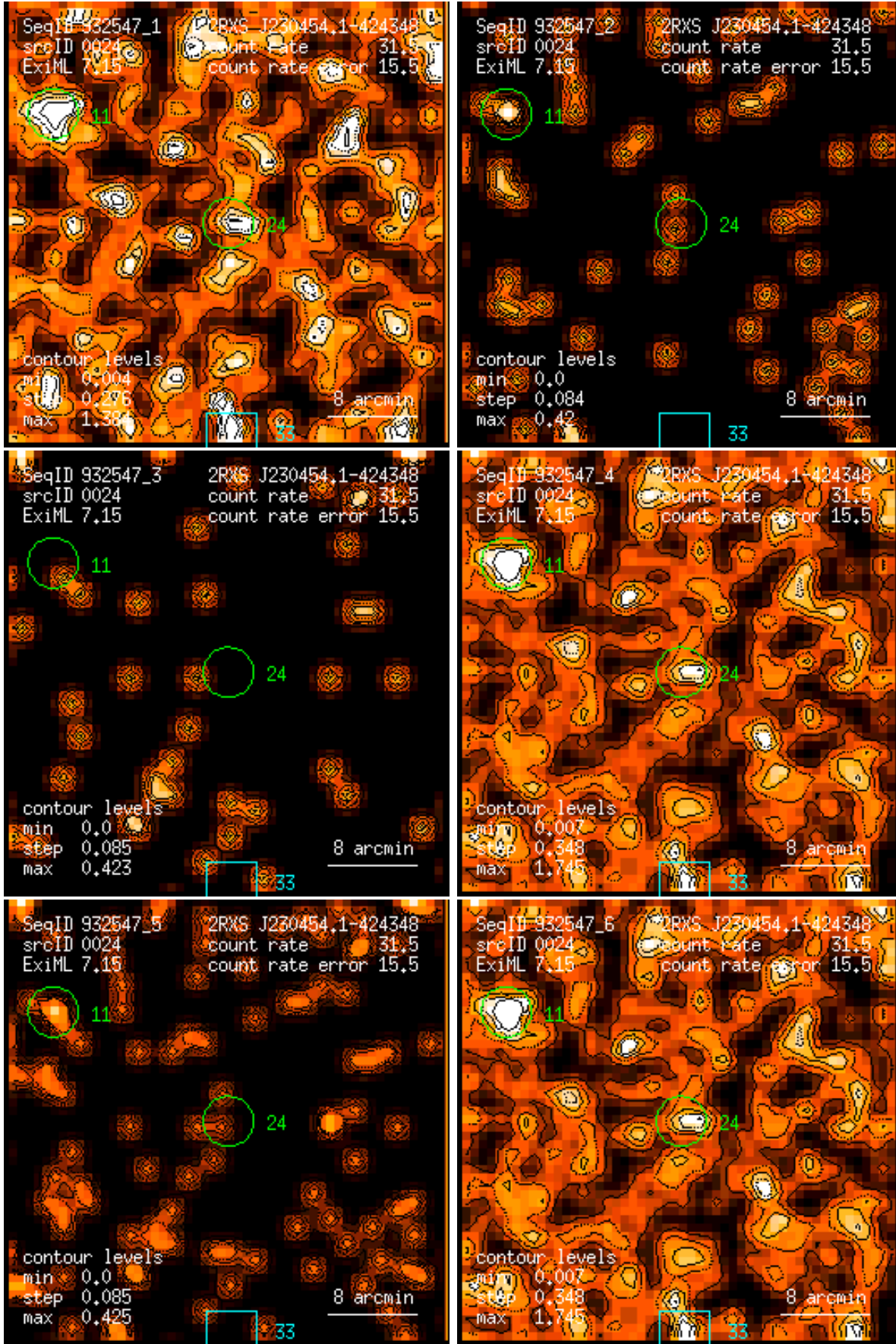
Figure 24: RASS 932547: detection 0024: band rate images, Gaussian filter: (1) PSPC channels 11 – 41, (2) 52 – 90, (3) 91 – 201, (4) 11 – 235, (5) 52 – 201, (6) 11 – 201. Broad band rates in counts/ks. Band rate contour levels in counts/ks/arcmin 2 .
