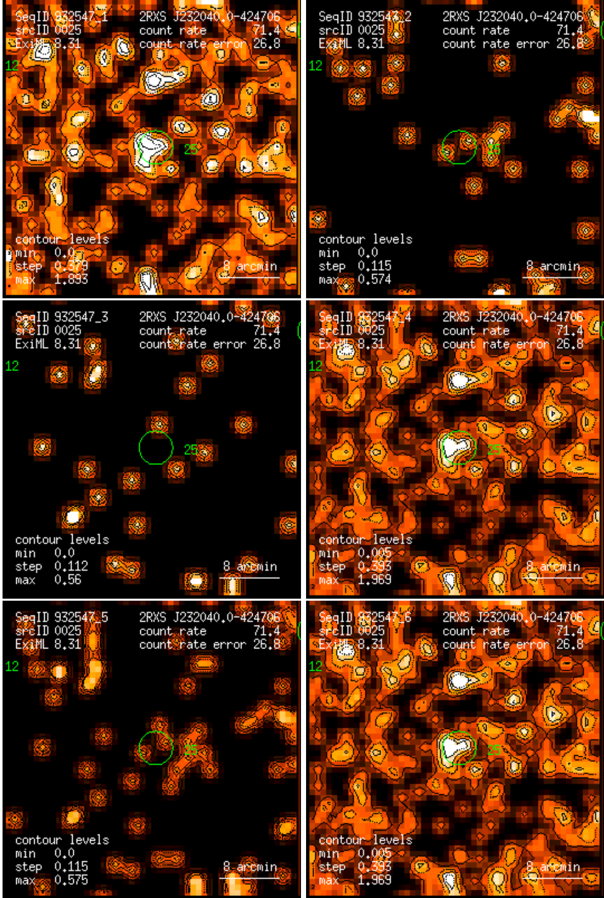
Figure 25: RASS 932547: detection 0025: band rate images, Gaussian filter: (1) PSPC channels 11 – 41, (2) 52 – 90, (3) 91 – 201, (4) 11 – 235, (5) 52 – 201, (6) 11 – 201. Broad band rates in counts/ks. Band rate contour levels in counts/ks/arcmin 2 .
