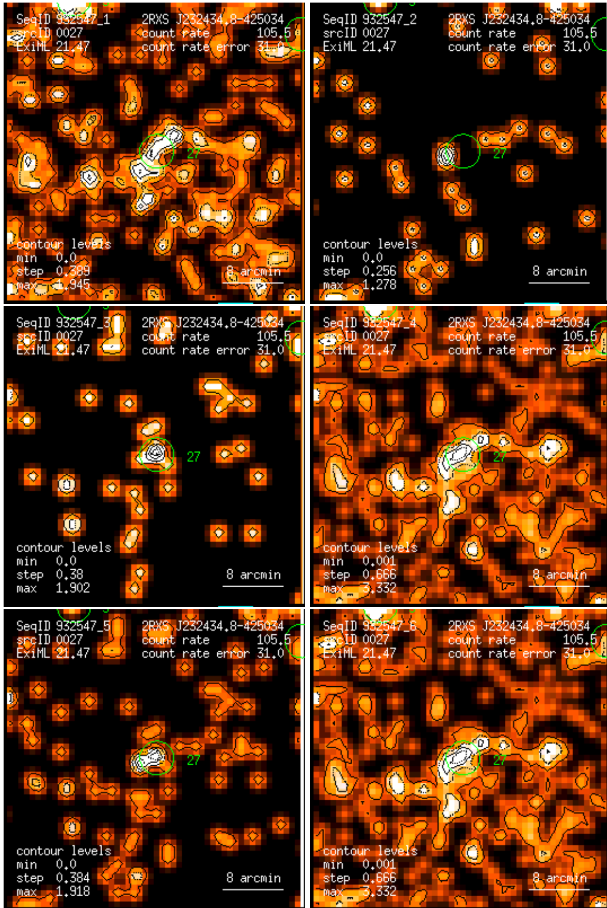
Figure 27: RASS 932547: detection 0027: band rate images, Gaussian filter: (1) PSPC channels 11 – 41, (2) 52 – 90, (3) 91 – 201, (4) 11 – 235, (5) 52 – 201, (6) 11 – 201. Broad band rates in counts/ks. Band rate contour levels in counts/ks/arcmin 2 .
