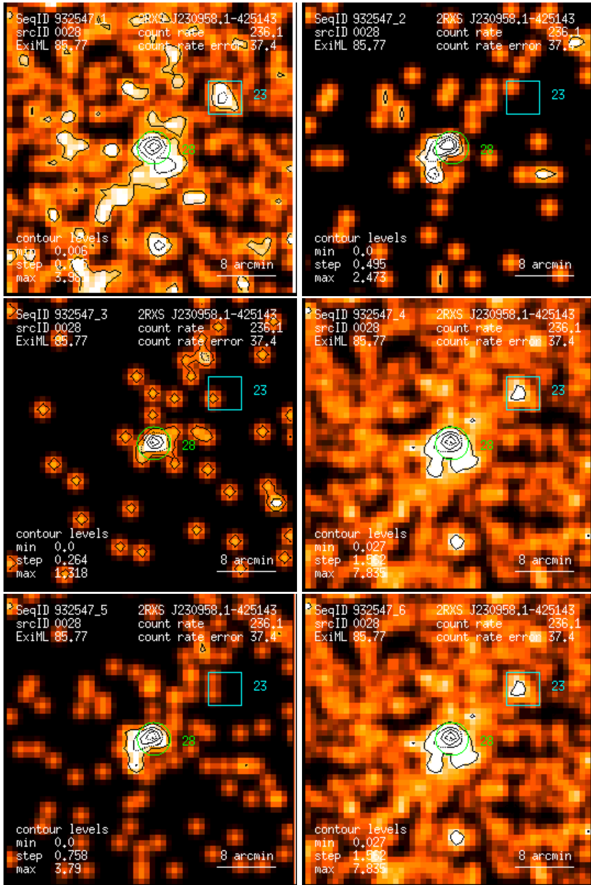
Figure 28: RASS 932547: detection 0028: band rate images, Gaussian filter: (1) PSPC channels 11 – 41, (2) 52 – 90, (3) 91 – 201, (4) 11 – 235, (5) 52 – 201, (6) 11 – 201. Broad band rates in counts/ks. Band rate contour levels in counts/ks/arcmin 2 .
