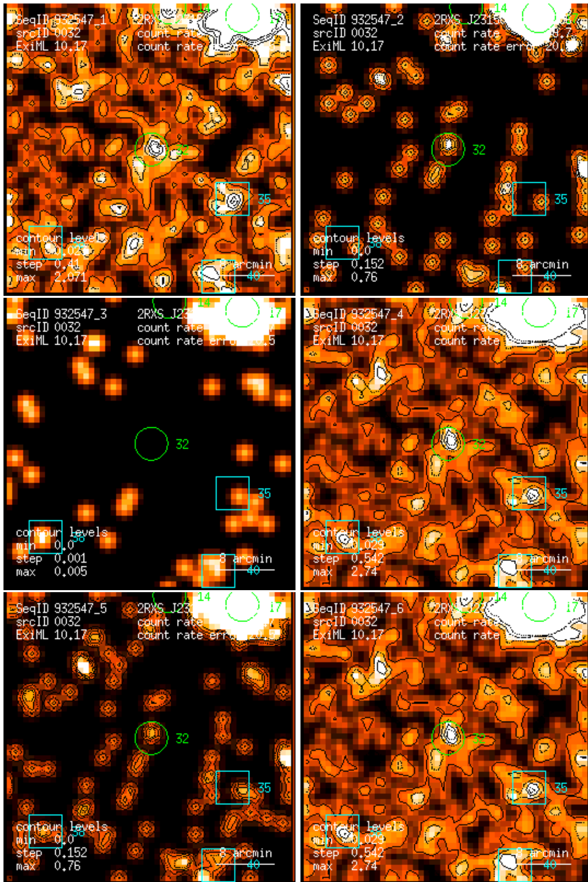
Figure 32: RASS 932547: detection 0032: band rate images, Gaussian filter: (1) PSPC channels 11 – 41, (2) 52 – 90, (3) 91 – 201, (4) 11 – 235, (5) 52 – 201, (6) 11 – 201. Broad band rates in counts/ks. Band rate contour levels in counts/ks/arcmin 2 .
