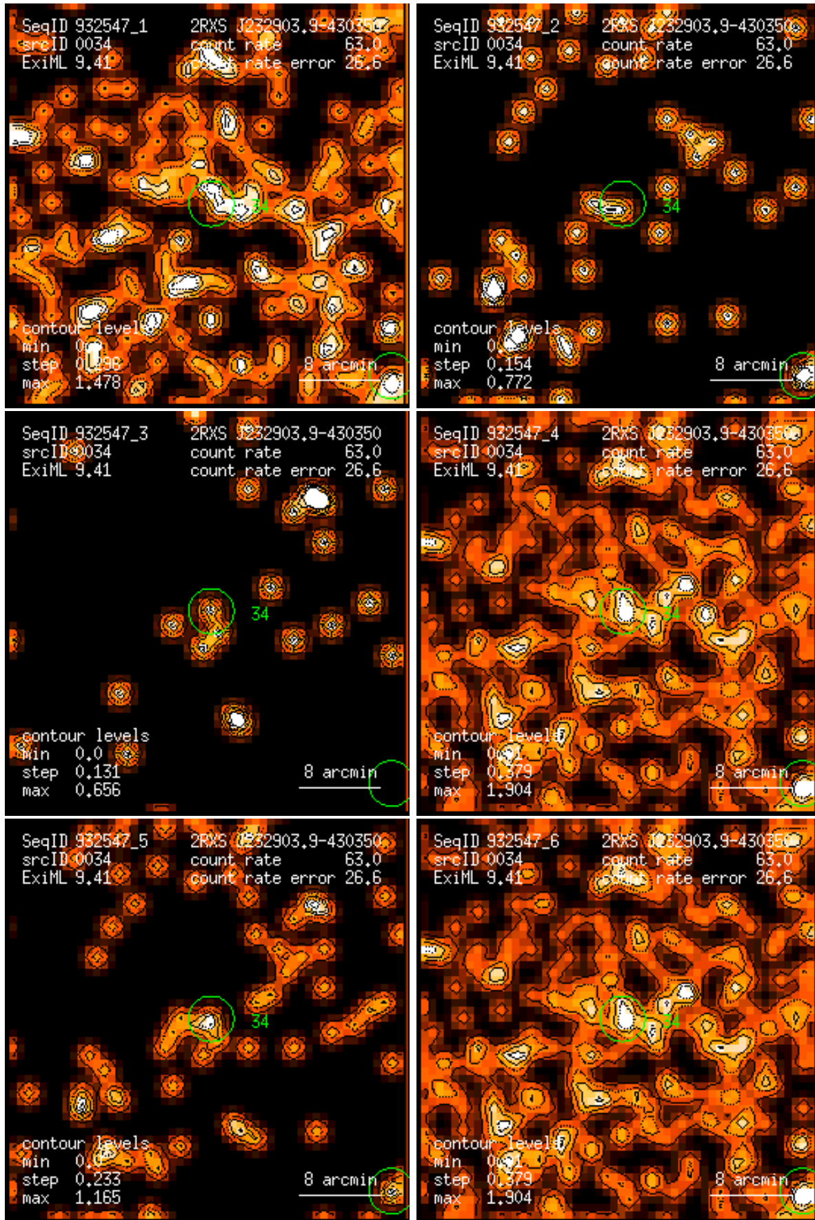
Figure 34: RASS 932547: detection 0034: band rate images, Gaussian filter: (1) PSPC channels 11 – 41, (2) 52 – 90, (3) 91 – 201, (4) 11 – 235, (5) 52 – 201, (6) 11 – 201. Broad band rates in counts/ks. Band rate contour levels in counts/ks/arcmin 2 .
