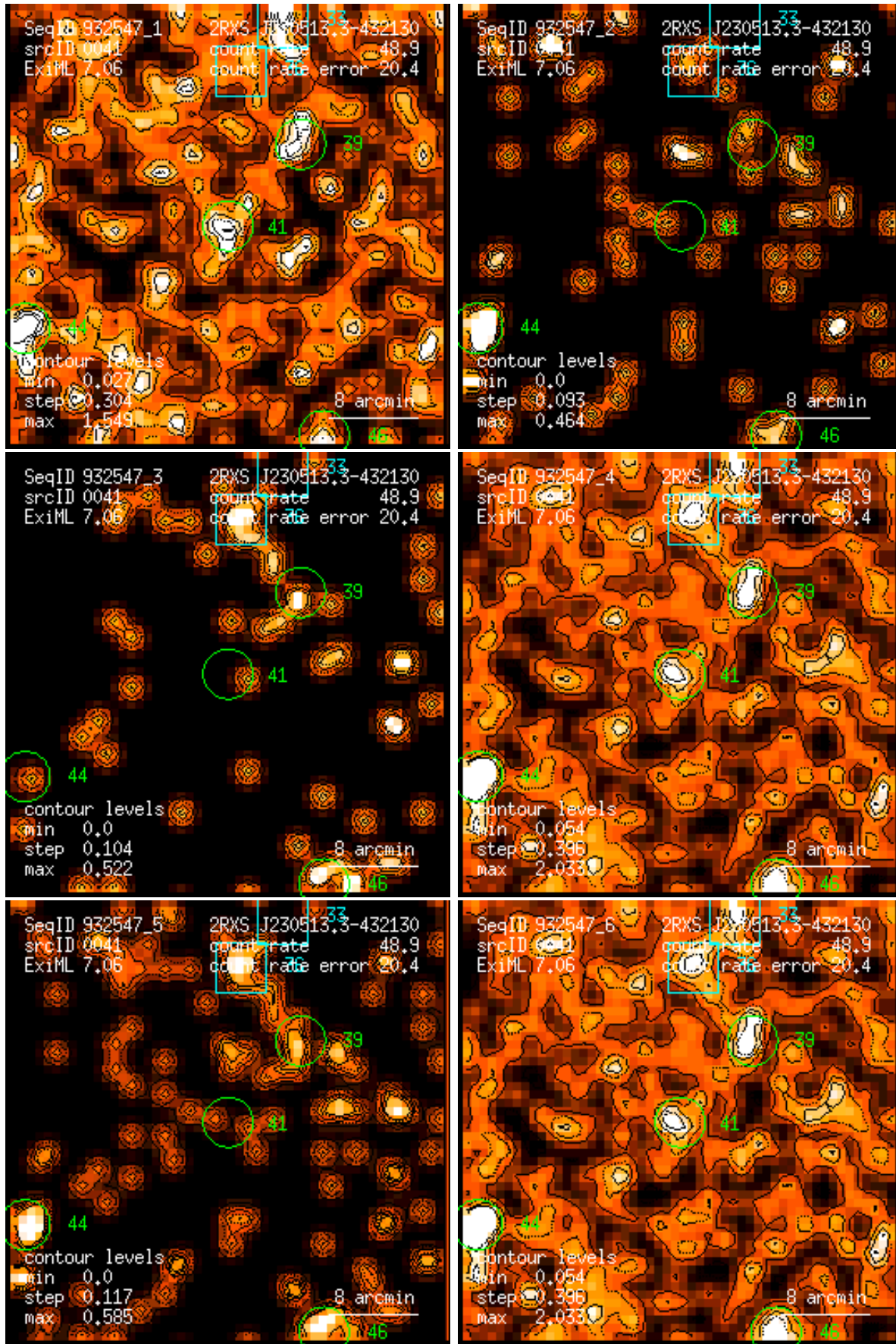
Figure 41: RASS 932547: detection 0041: band rate images, Gaussian filter: (1) PSPC channels 11 – 41, (2) 52 – 90, (3) 91 – 201, (4) 11 – 235, (5) 52 – 201, (6) 11 – 201. Broad band rates in counts/ks. Band rate contour levels in counts/ks/arcmin 2 .
