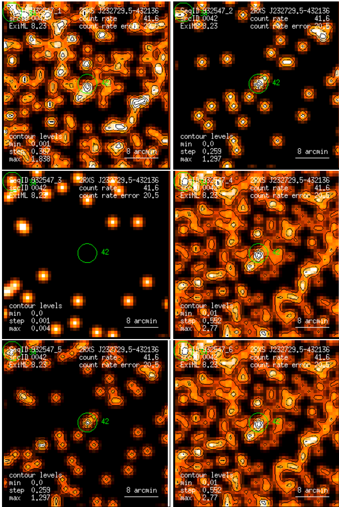
Figure 42: RASS 932547: detection 0042: band rate images, Gaussian filter: (1) PSPC channels 11 – 41, (2) 52 – 90, (3) 91 – 201, (4) 11 – 235, (5) 52 – 201, (6) 11 – 201. Broad band rates in counts/ks. Band rate contour levels in counts/ks/arcmin 2 .
