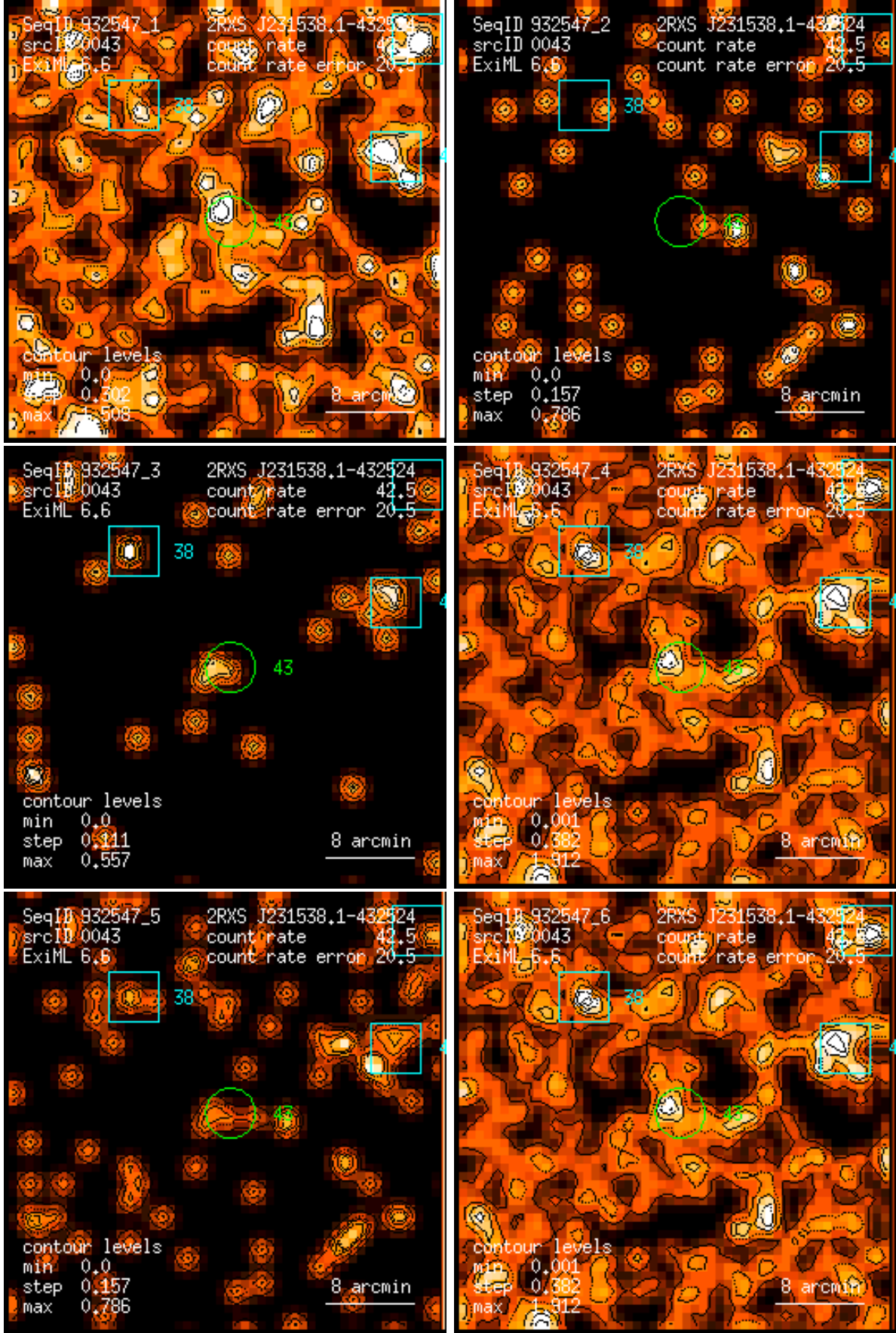
Figure 43: RASS 932547: detection 0043: band rate images, Gaussian filter: (1) PSPC channels 11 – 41, (2) 52 – 90, (3) 91 – 201, (4) 11 – 235, (5) 52 – 201, (6) 11 – 201. Broad band rates in counts/ks. Band rate contour levels in counts/ks/arcmin 2 .
