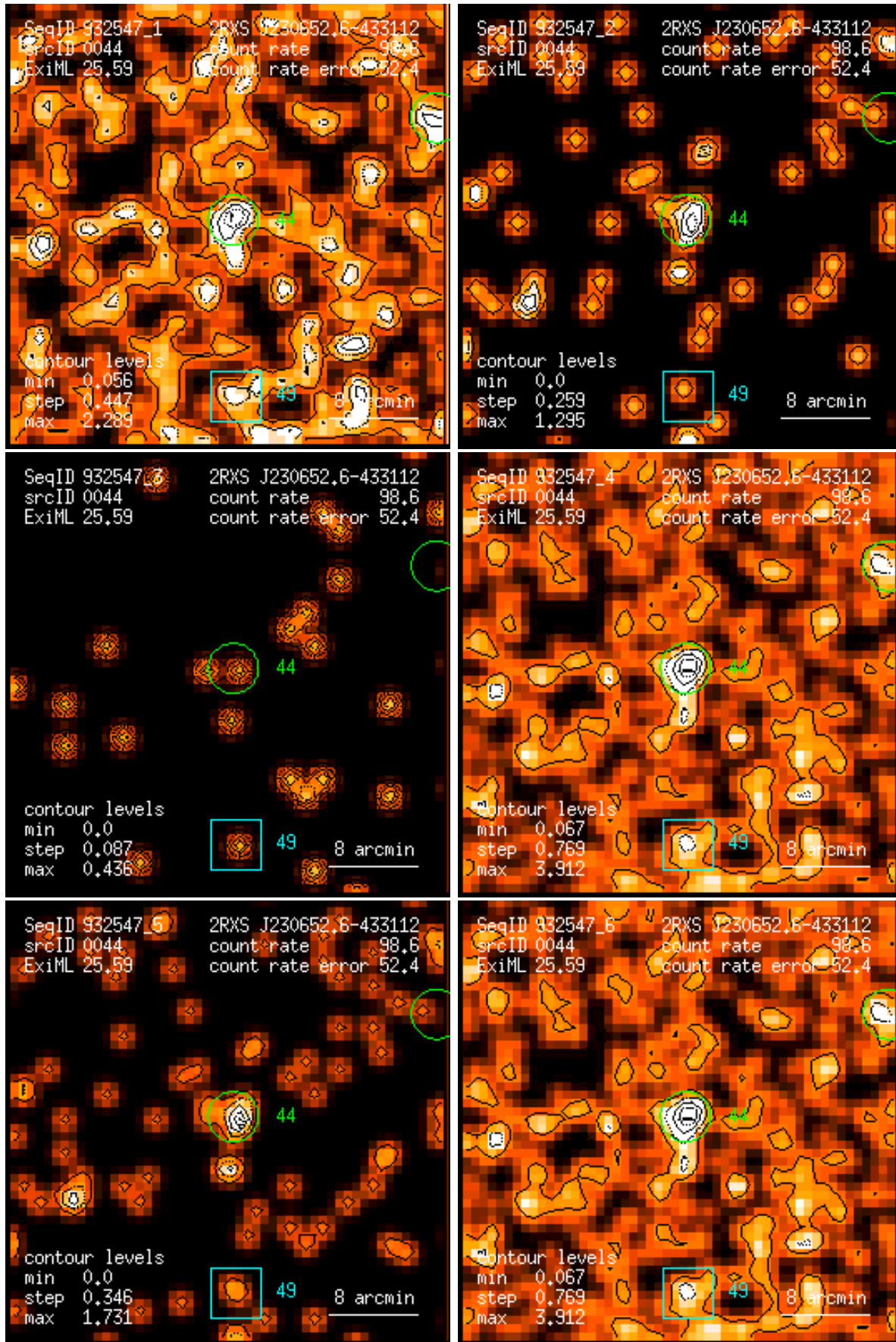
Figure 44: RASS 932547: detection 0044: band rate images, Gaussian filter: (1) PSPC channels 11 – 41, (2) 52 – 90, (3) 91 – 201, (4) 11 – 235, (5) 52 – 201, (6) 11 – 201. Broad band rates in counts/ks. Band rate contour levels in counts/ks/arcmin 2 .
