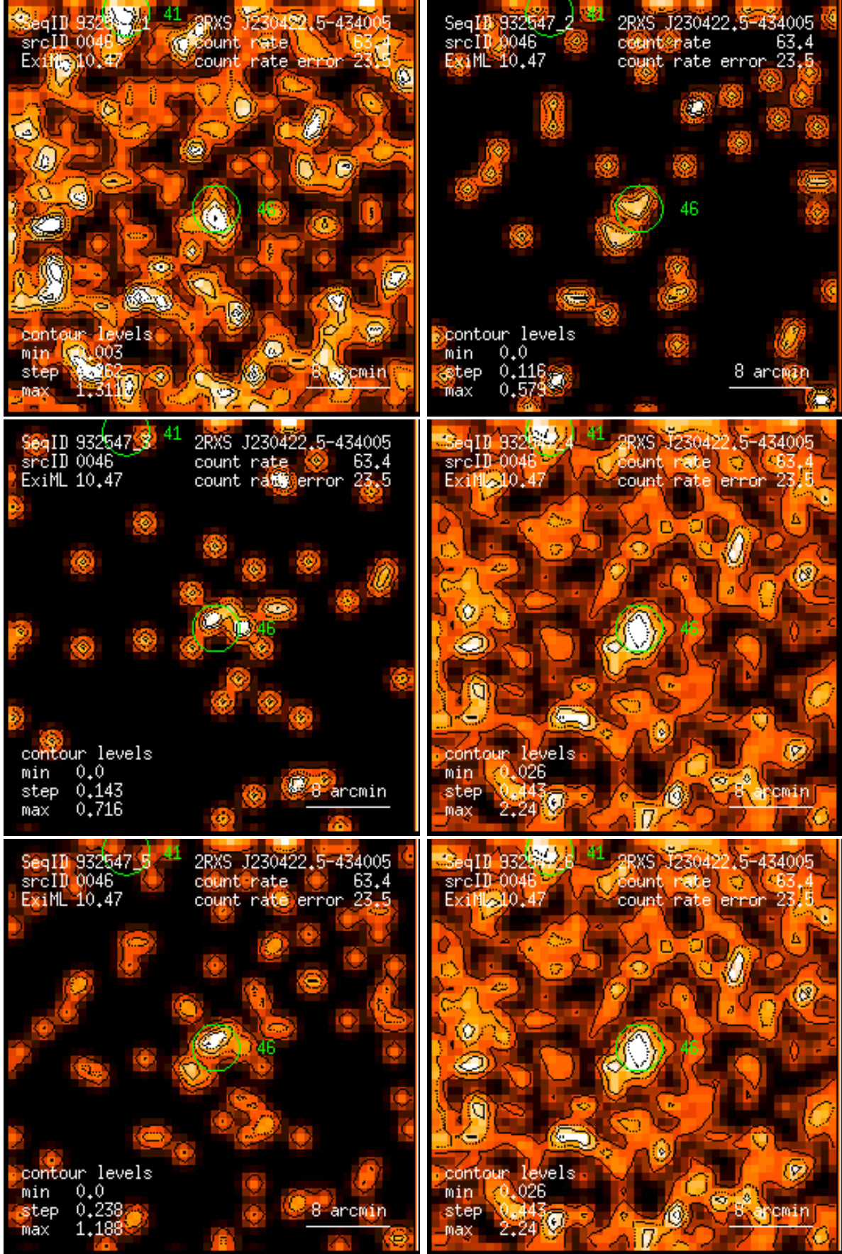
Figure 46: RASS 932547: detection 0046: band rate images, Gaussian filter: (1) PSPC channels 11 – 41, (2) 52 – 90, (3) 91 – 201, (4) 11 – 235, (5) 52 – 201, (6) 11 – 201. Broad band rates in counts/ks. Band rate contour levels in counts/ks/arcmin 2 .
