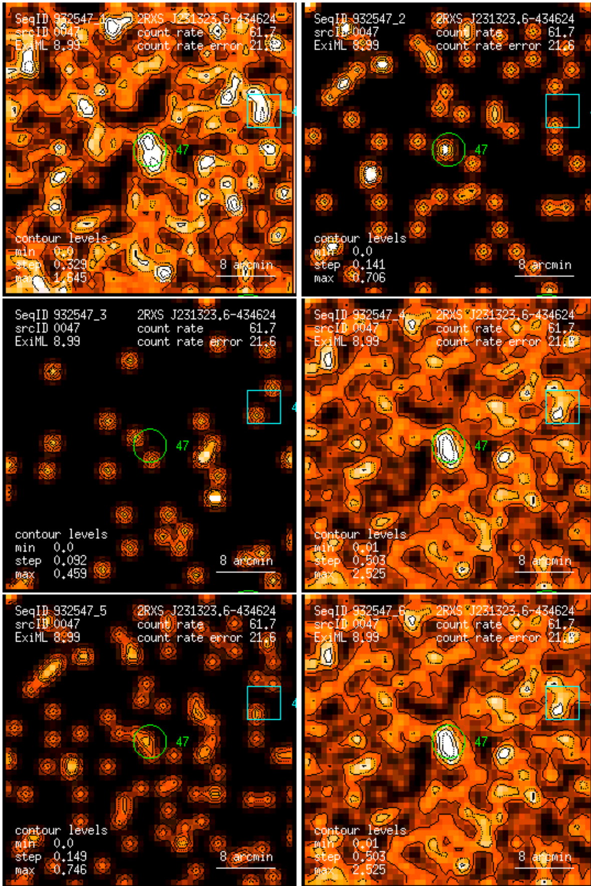
Figure 47: RASS 932547: detection 0047: band rate images, Gaussian filter: (1) PSPC channels 11 – 41, (2) 52 – 90, (3) 91 – 201, (4) 11 – 235, (5) 52 – 201, (6) 11 – 201. Broad band rates in counts/ks. Band rate contour levels in counts/ks/arcmin 2 .
