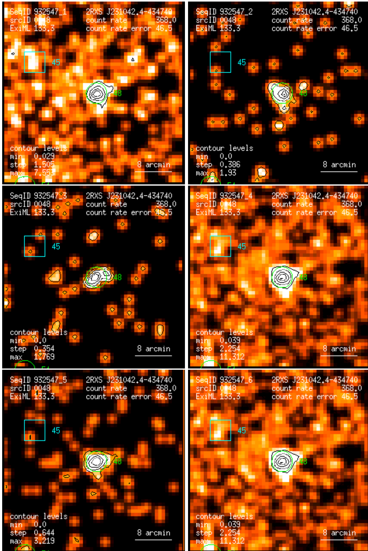
Figure 48: RASS 932547: detection 0048: band rate images, Gaussian filter: (1) PSPC channels 11 – 41, (2) 52 – 90, (3) 91 – 201, (4) 11 – 235, (5) 52 – 201, (6) 11 – 201. Broad band rates in counts/ks. Band rate contour levels in counts/ks/arcmin 2 .
