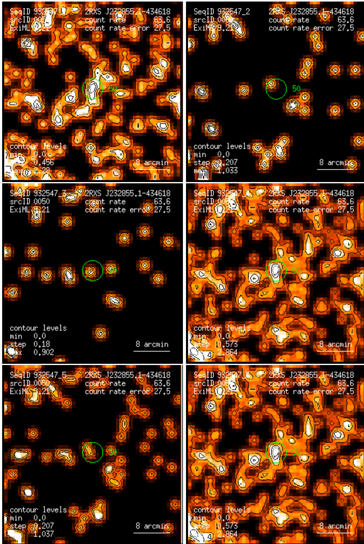
Figure 50: RASS 932547: detection 0050: band rate images, Gaussian filter: (1) PSPC channels 11 – 41, (2) 52 – 90, (3) 91 – 201, (4) 11 – 235, (5) 52 – 201, (6) 11 – 201. Broad band rates in counts/ks. Band rate contour levels in counts/ks/arcmin 2 .
