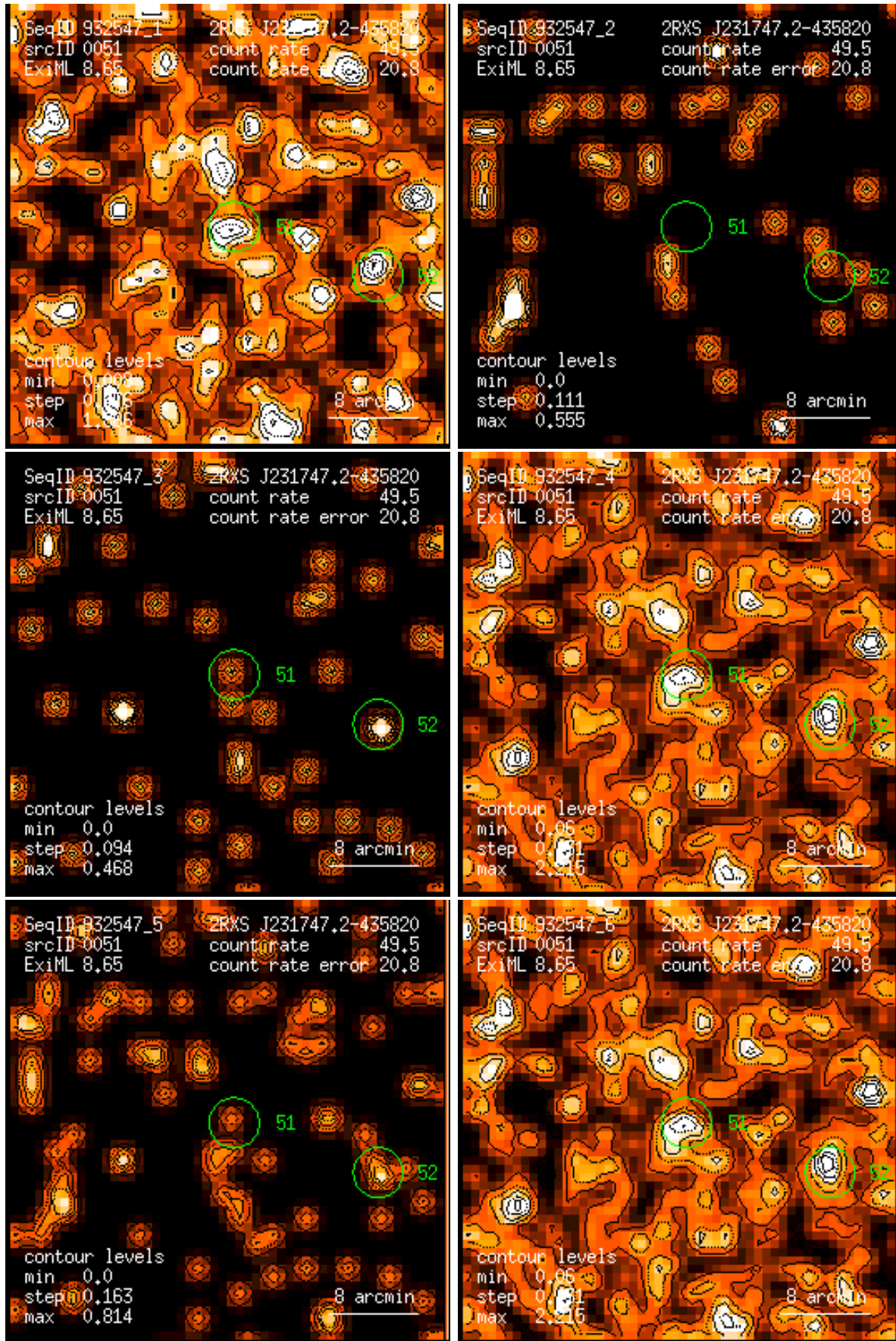
Figure 51: RASS 932547: detection 0051: band rate images, Gaussian filter: (1) PSPC channels 11 – 41, (2) 52 – 90, (3) 91 – 201, (4) 11 – 235, (5) 52 – 201, (6) 11 – 201. Broad band rates in counts/ks. Band rate contour levels in counts/ks/arcmin 2 .
