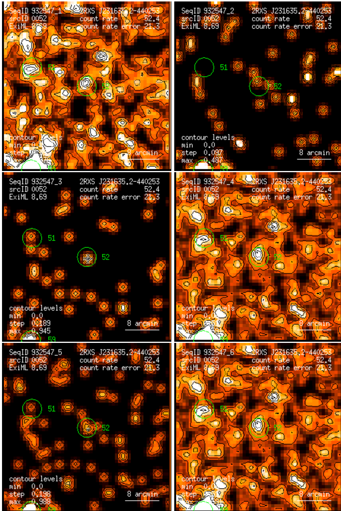
Figure 52: RASS 932547: detection 0052: band rate images, Gaussian filter: (1) PSPC channels 11 – 41, (2) 52 – 90, (3) 91 – 201, (4) 11 – 235, (5) 52 – 201, (6) 11 – 201. Broad band rates in counts/ks. Band rate contour levels in counts/ks/arcmin 2 .
