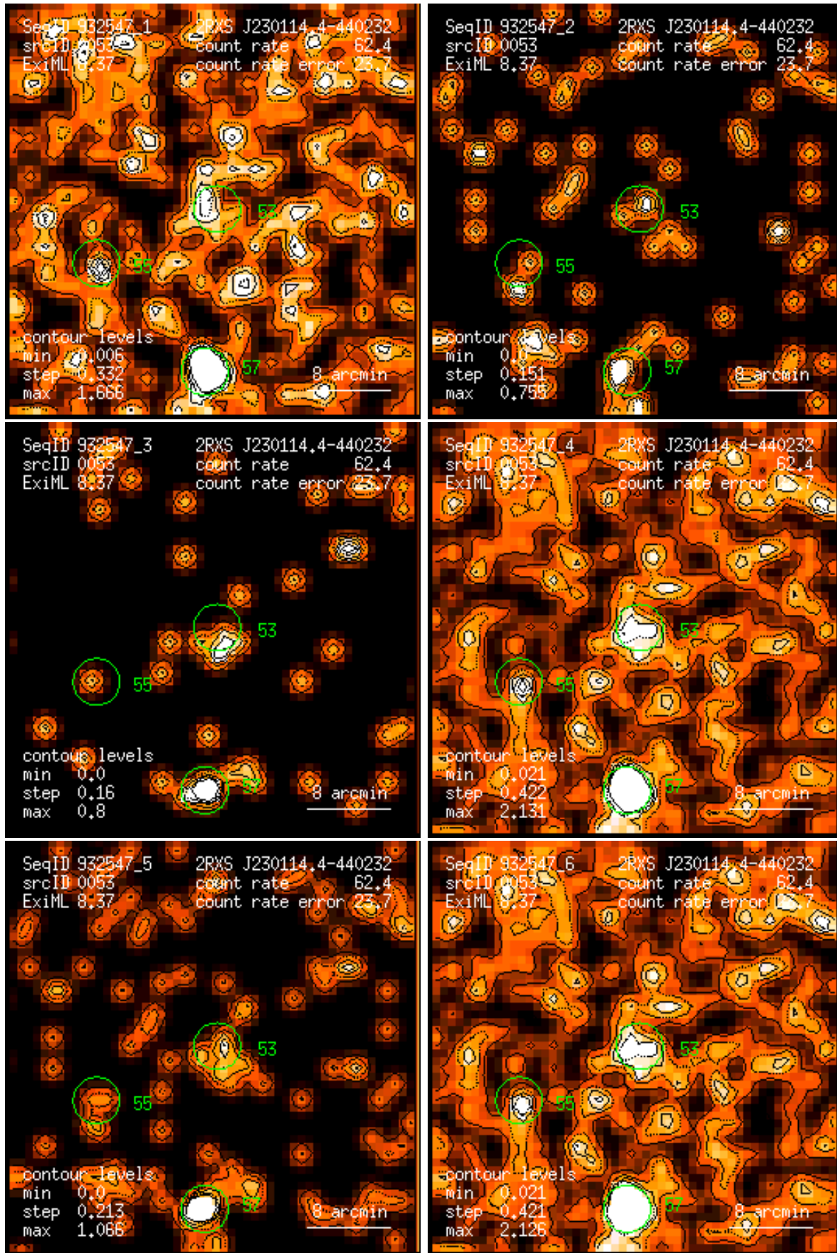
Figure 53: RASS 932547: detection 0053: band rate images, Gaussian filter: (1) PSPC channels 11 – 41, (2) 52 – 90, (3) 91 – 201, (4) 11 – 235, (5) 52 – 201, (6) 11 – 201. Broad band rates in counts/ks. Band rate contour levels in counts/ks/arcmin 2 .
