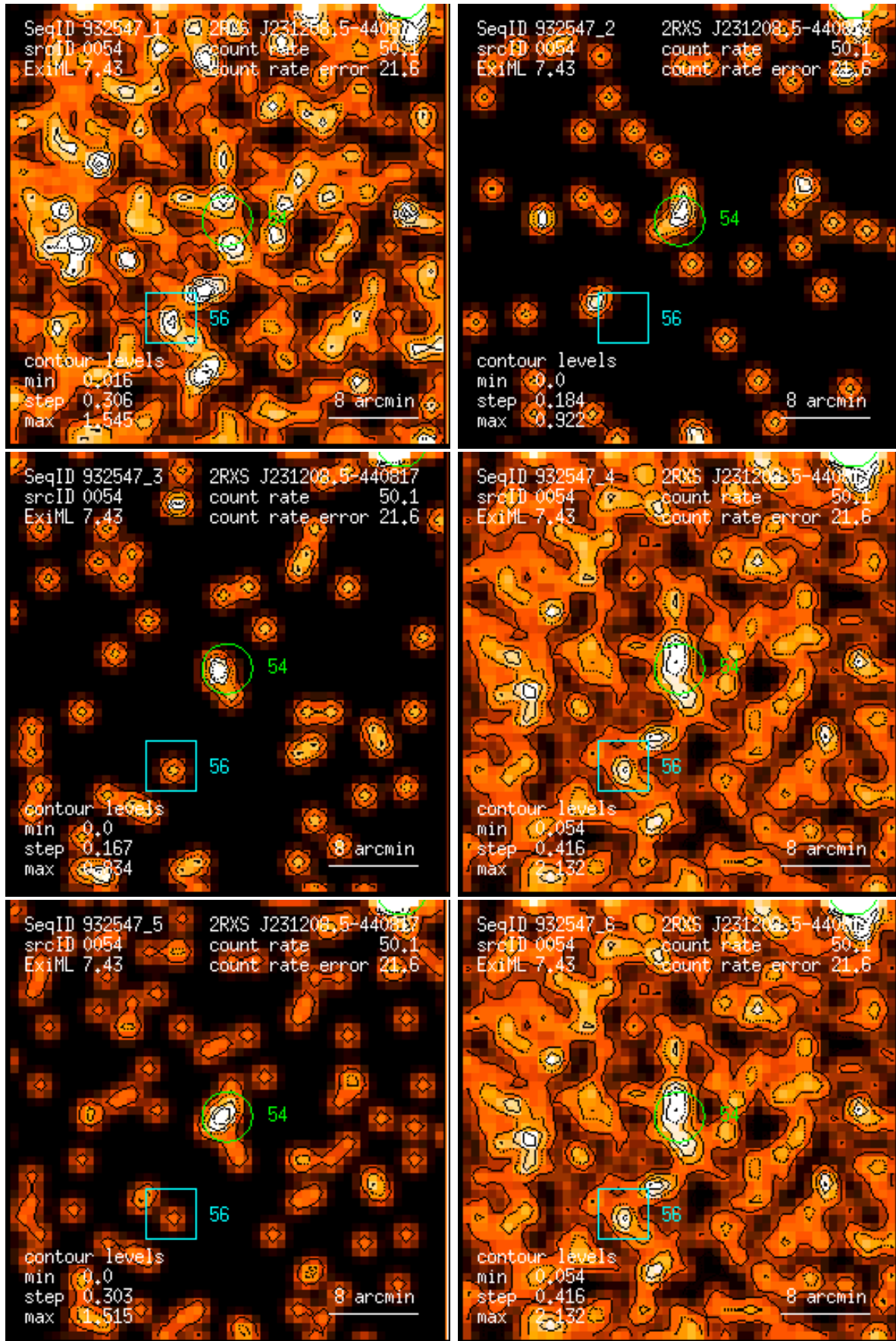
Figure 54: RASS 932547: detection 0054: band rate images, Gaussian filter: (1) PSPC channels 11 – 41, (2) 52 – 90, (3) 91 – 201, (4) 11 – 235, (5) 52 – 201, (6) 11 – 201. Broad band rates in counts/ks. Band rate contour levels in counts/ks/arcmin 2 .
