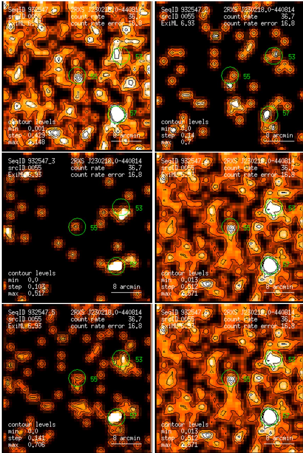
Figure 55: RASS 932547: detection 0055: band rate images, Gaussian filter: (1) PSPC channels 11 – 41, (2) 52 – 90, (3) 91 – 201, (4) 11 – 235, (5) 52 – 201, (6) 11 – 201. Broad band rates in counts/ks. Band rate contour levels in counts/ks/arcmin 2 .
