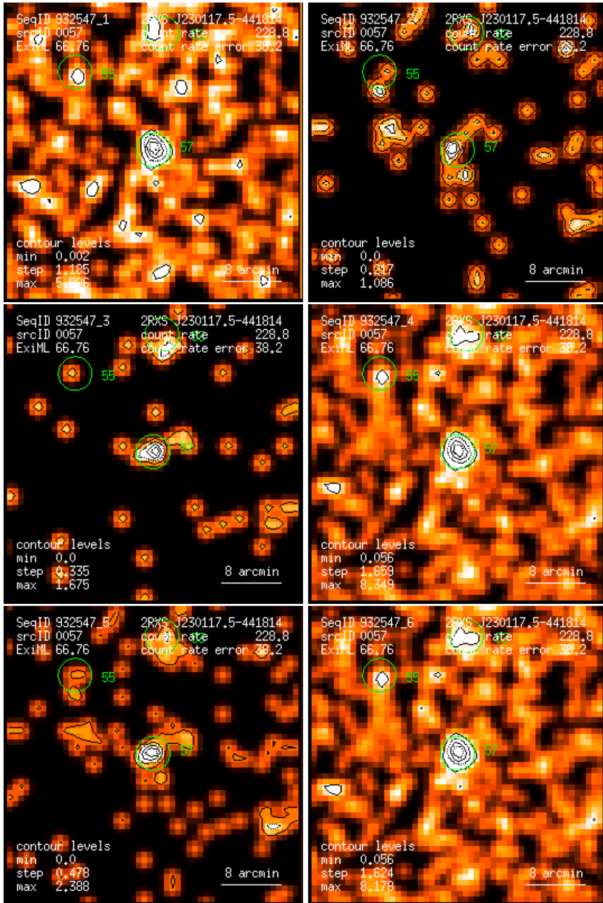
Figure 57: RASS 932547: detection 0057: band rate images, Gaussian filter: (1) PSPC channels 11 – 41, (2) 52 – 90, (3) 91 – 201, (4) 11 – 235, (5) 52 – 201, (6) 11 – 201. Broad band rates in counts/ks. Band rate contour levels in counts/ks/arcmin 2 .
