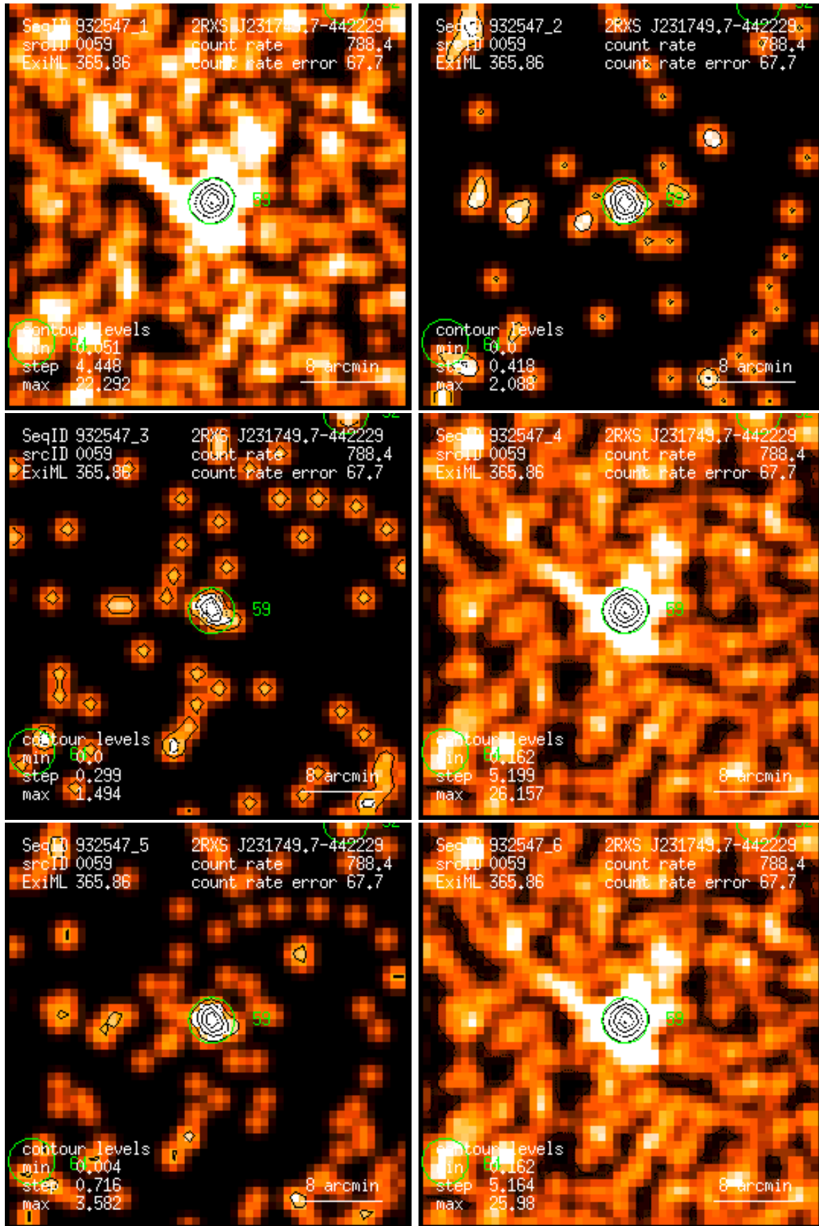
Figure 59: RASS 932547: detection 0059: band rate images, Gaussian filter: (1) PSPC channels 11 – 41, (2) 52 – 90, (3) 91 – 201, (4) 11 – 235, (5) 52 – 201, (6) 11 – 201. Broad band rates in counts/ks. Band rate contour levels in counts/ks/arcmin 2 .
