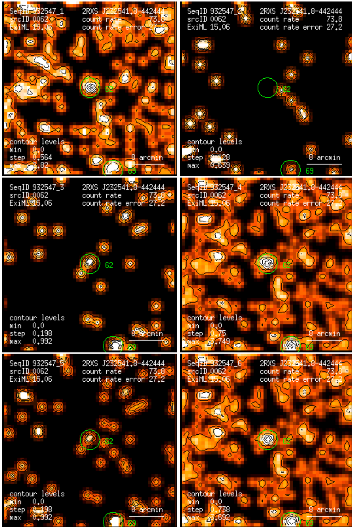
Figure 62: RASS 932547: detection 0062: band rate images, Gaussian filter: (1) PSPC channels 11 – 41, (2) 52 – 90, (3) 91 – 201, (4) 11 – 235, (5) 52 – 201, (6) 11 – 201. Broad band rates in counts/ks. Band rate contour levels in counts/ks/arcmin 2 .
