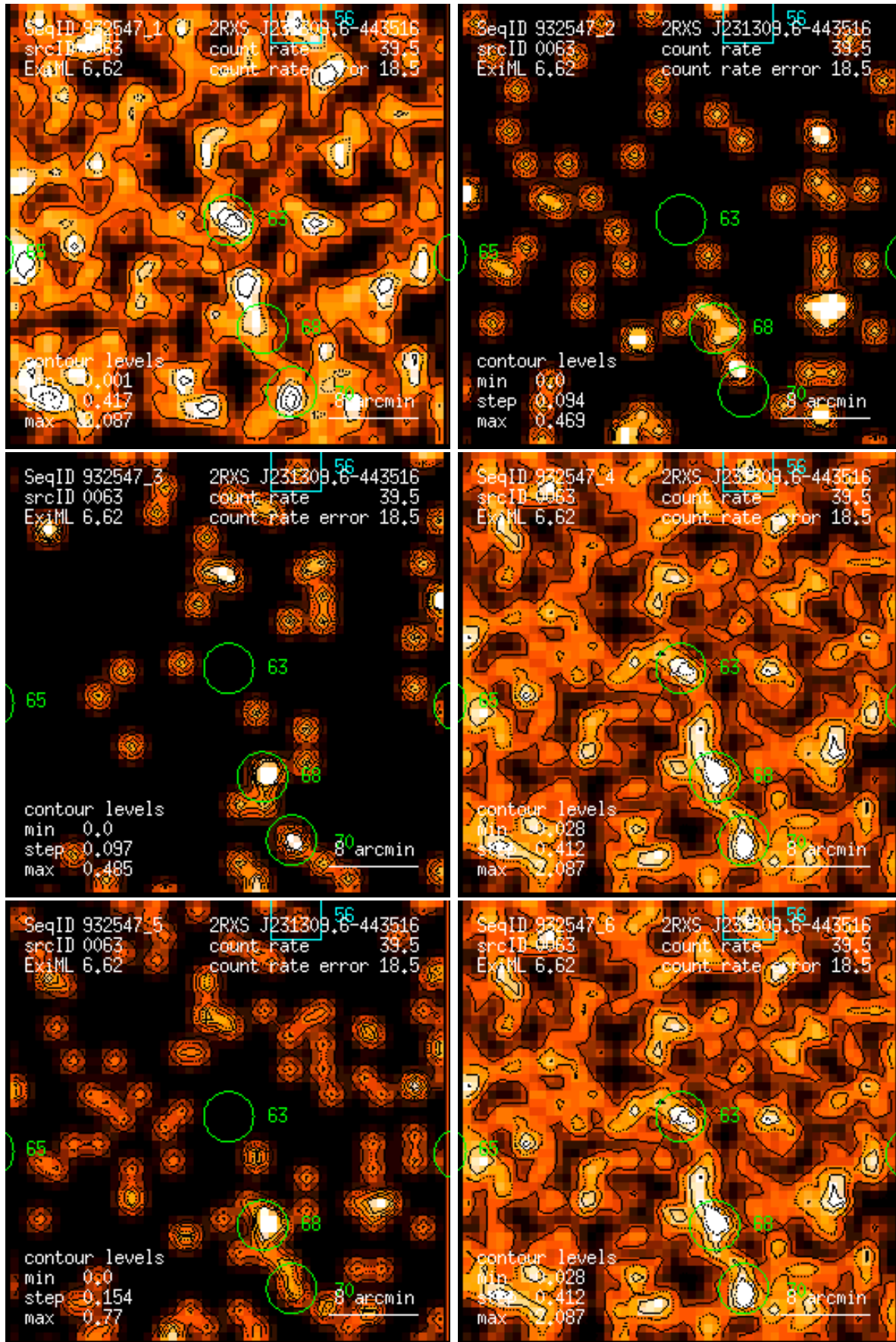
Figure 63: RASS 932547: detection 0063: band rate images, Gaussian filter: (1) PSPC channels 11 – 41, (2) 52 – 90, (3) 91 – 201, (4) 11 – 235, (5) 52 – 201, (6) 11 – 201. Broad band rates in counts/ks. Band rate contour levels in counts/ks/arcmin 2 .
