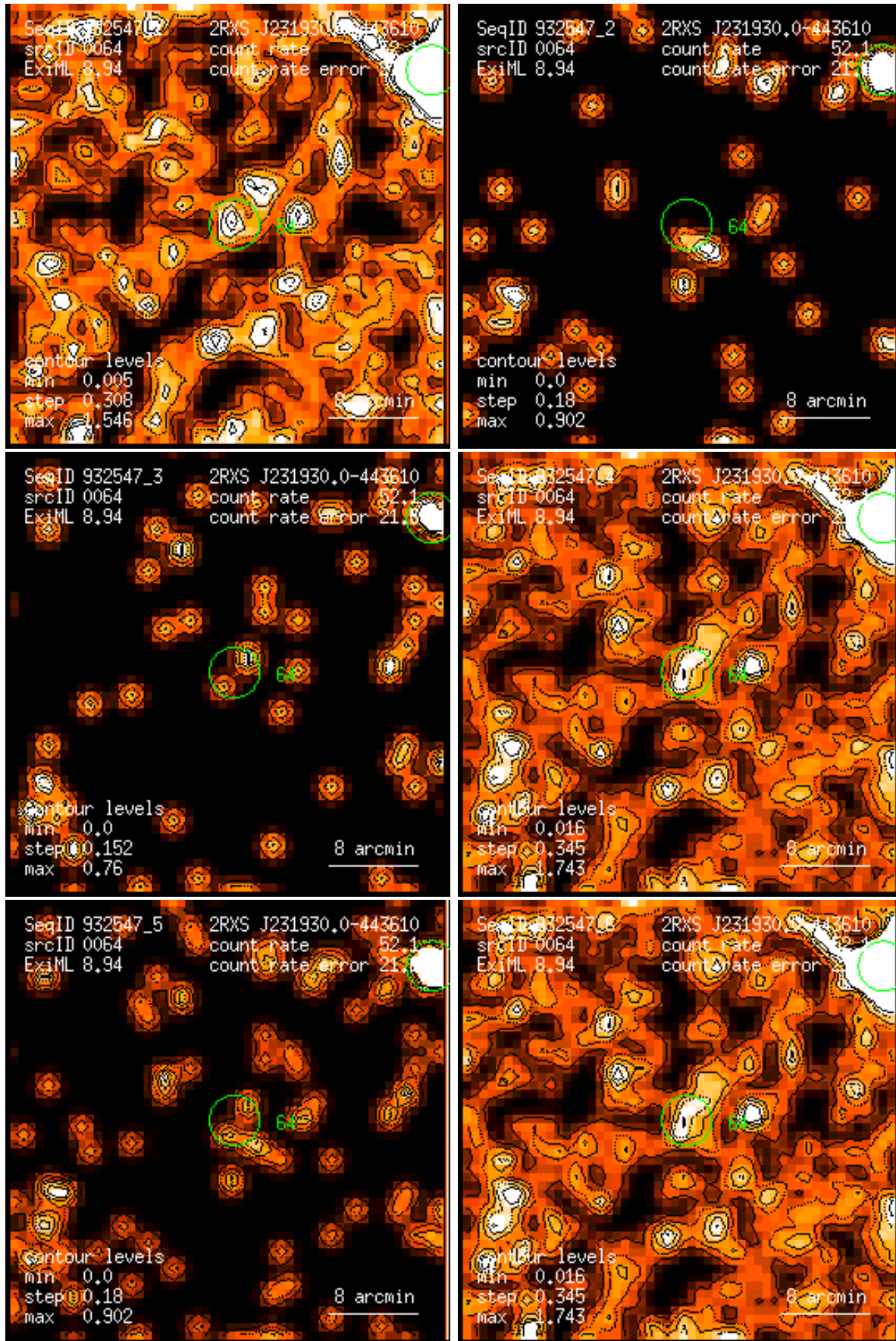
Figure 64: RASS 932547: detection 0064: band rate images, Gaussian filter: (1) PSPC channels 11 – 41, (2) 52 – 90, (3) 91 – 201, (4) 11 – 235, (5) 52 – 201, (6) 11 – 201. Broad band rates in counts/ks. Band rate contour levels in counts/ks/arcmin 2 .
