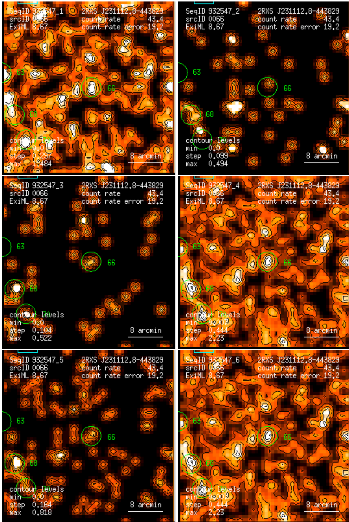
Figure 66: RASS 932547: detection 0066: band rate images, Gaussian filter: (1) PSPC channels 11 – 41, (2) 52 – 90, (3) 91 – 201, (4) 11 – 235, (5) 52 – 201, (6) 11 – 201. Broad band rates in counts/ks. Band rate contour levels in counts/ks/arcmin 2 .
