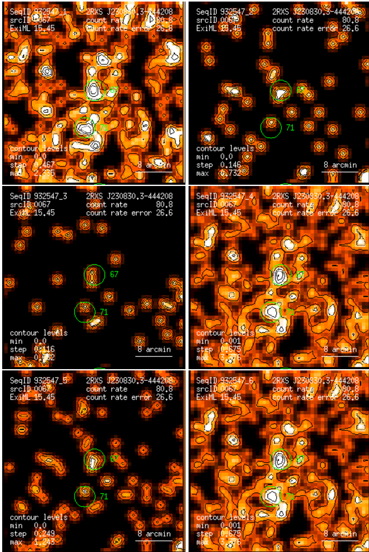
Figure 67: RASS 932547: detection 0067: band rate images, Gaussian filter: (1) PSPC channels 11 – 41, (2) 52 – 90, (3) 91 – 201, (4) 11 – 235, (5) 52 – 201, (6) 11 – 201. Broad band rates in counts/ks. Band rate contour levels in counts/ks/arcmin 2 .
