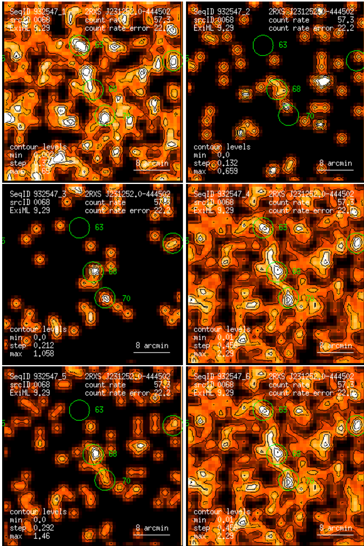
Figure 68: RASS 932547: detection 0068: band rate images, Gaussian filter: (1) PSPC channels 11 – 41, (2) 52 – 90, (3) 91 – 201, (4) 11 – 235, (5) 52 – 201, (6) 11 – 201. Broad band rates in counts/ks. Band rate contour levels in counts/ks/arcmin 2 .
