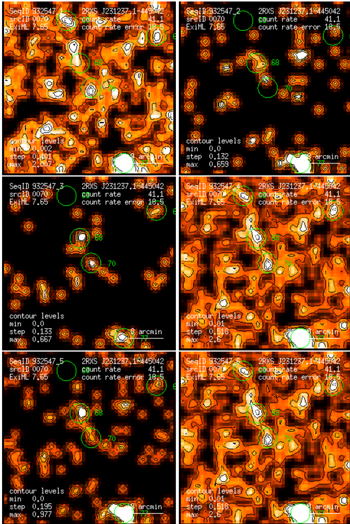
Figure 70: RASS 932547: detection 0070: band rate images, Gaussian filter: (1) PSPC channels 11 – 41, (2) 52 – 90, (3) 91 – 201, (4) 11 – 235, (5) 52 – 201, (6) 11 – 201. Broad band rates in counts/ks. Band rate contour levels in counts/ks/arcmin 2 .
