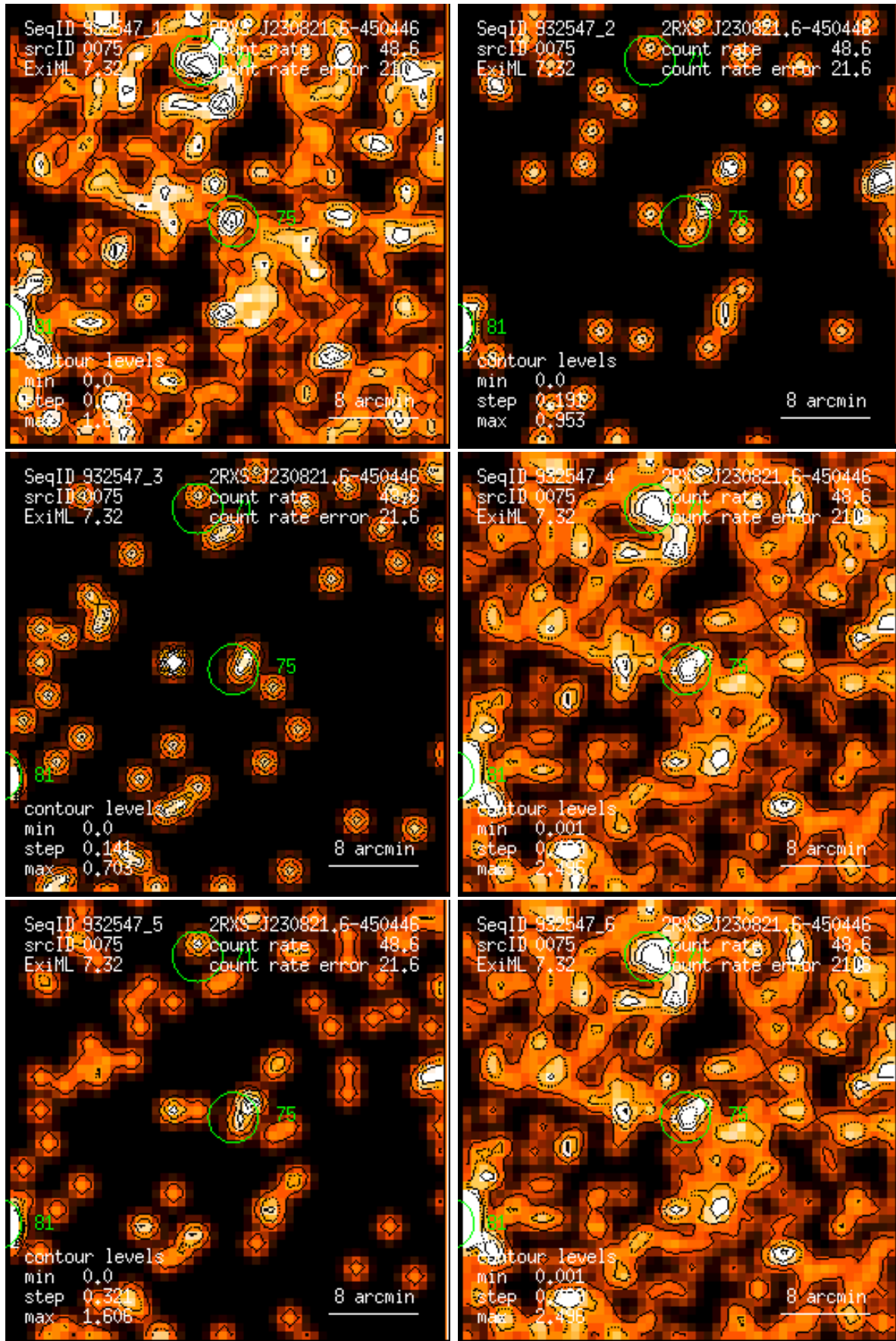
Figure 75: RASS 932547: detection 0075: band rate images, Gaussian filter: (1) PSPC channels 11 – 41, (2) 52 – 90, (3) 91 – 201, (4) 11 – 235, (5) 52 – 201, (6) 11 – 201. Broad band rates in counts/ks. Band rate contour levels in counts/ks/arcmin 2 .
