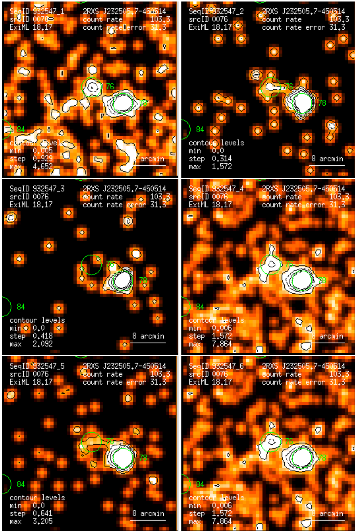
Figure 76: RASS 932547: detection 0076: band rate images, Gaussian filter: (1) PSPC channels 11 – 41, (2) 52 – 90, (3) 91 – 201, (4) 11 – 235, (5) 52 – 201, (6) 11 – 201. Broad band rates in counts/ks. Band rate contour levels in counts/ks/arcmin 2 .
