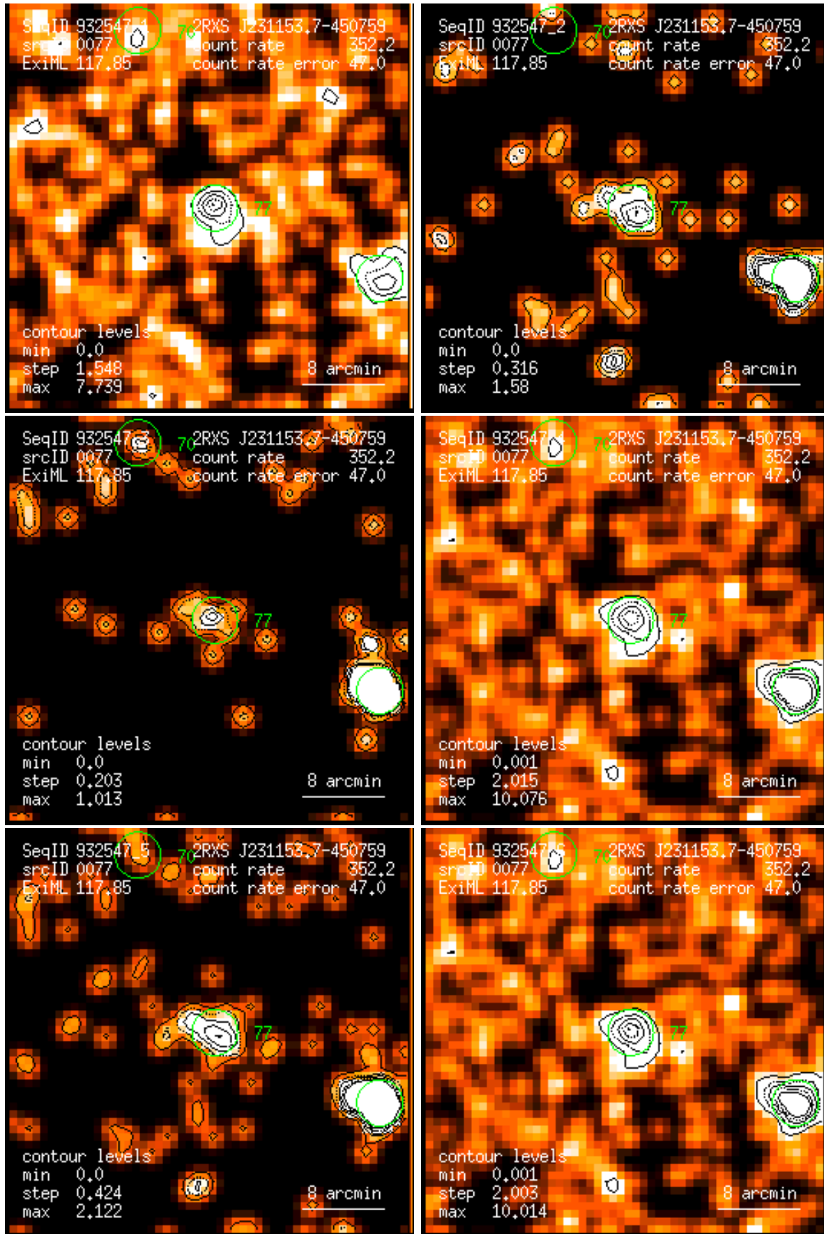
Figure 77: RASS 932547: detection 0077: band rate images, Gaussian filter: (1) PSPC channels 11 – 41, (2) 52 – 90, (3) 91 – 201, (4) 11 – 235, (5) 52 – 201, (6) 11 – 201. Broad band rates in counts/ks. Band rate contour levels in counts/ks/arcmin 2 .
