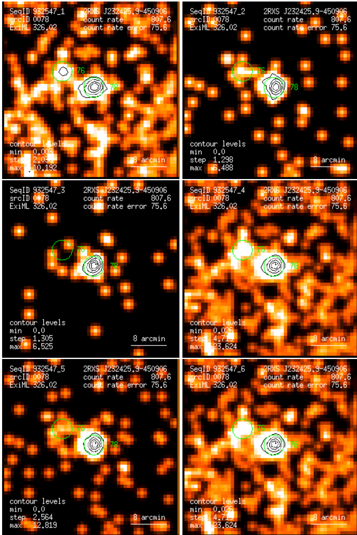
Figure 78: RASS 932547: detection 0078: band rate images, Gaussian filter: (1) PSPC channels 11 – 41, (2) 52 – 90, (3) 91 – 201, (4) 11 – 235, (5) 52 – 201, (6) 11 – 201. Broad band rates in counts/ks. Band rate contour levels in counts/ks/arcmin 2 .
