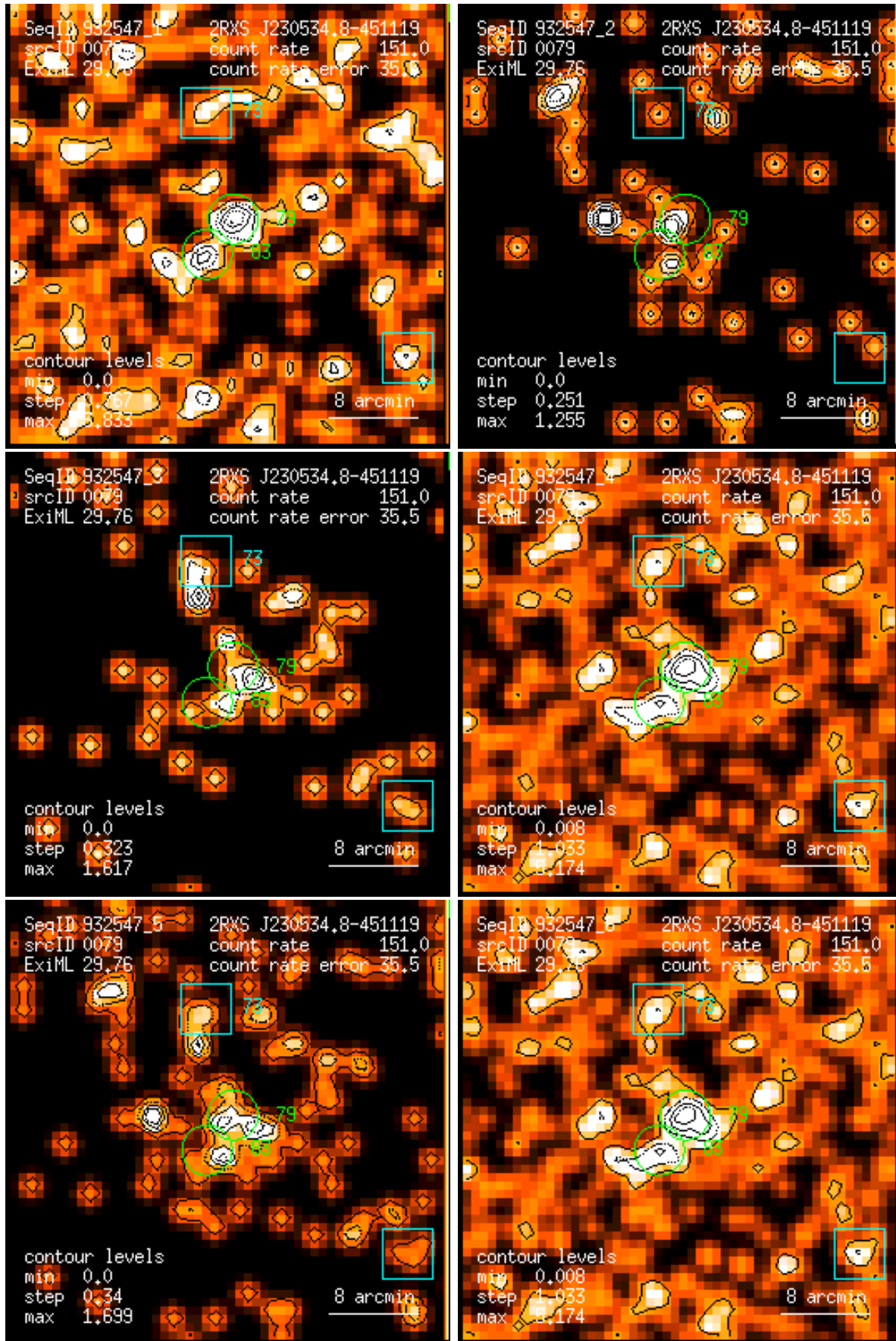
Figure 79: RASS 932547: detection 0079: band rate images, Gaussian filter: (1) PSPC channels 11 – 41, (2) 52 – 90, (3) 91 – 201, (4) 11 – 235, (5) 52 – 201, (6) 11 – 201. Broad band rates in counts/ks. Band rate contour levels in counts/ks/arcmin 2 .
