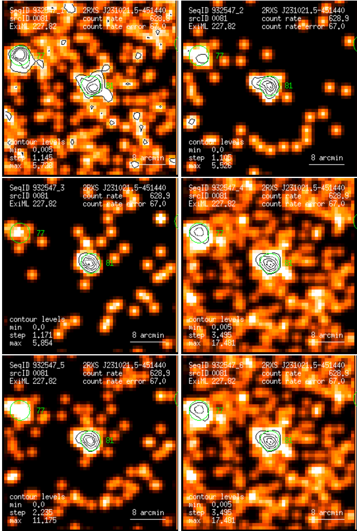
Figure 81: RASS 932547: detection 0081: band rate images, Gaussian filter: (1) PSPC channels 11 – 41, (2) 52 – 90, (3) 91 – 201, (4) 11 – 235, (5) 52 – 201, (6) 11 – 201. Broad band rates in counts/ks. Band rate contour levels in counts/ks/arcmin 2 .
