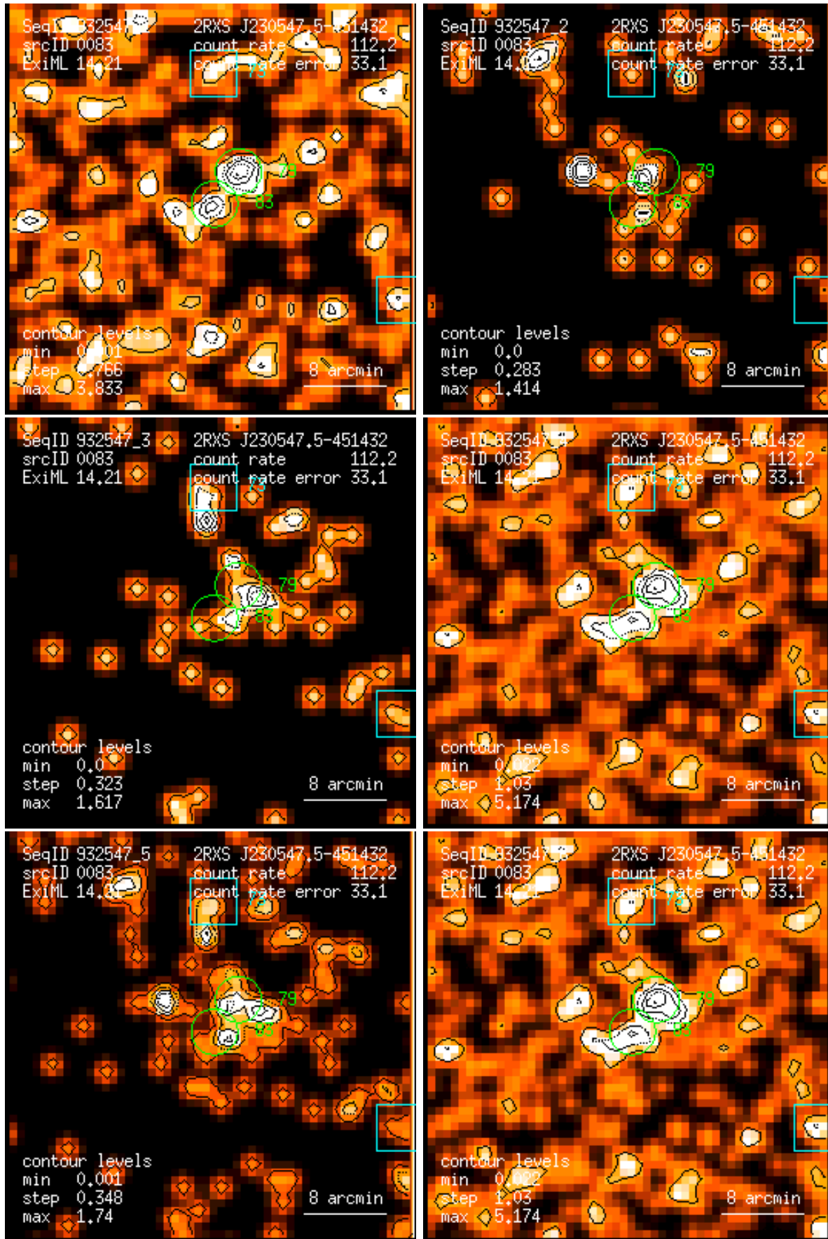
Figure 83: RASS 932547: detection 0083: band rate images, Gaussian filter: (1) PSPC channels 11 – 41, (2) 52 – 90, (3) 91 – 201, (4) 11 – 235, (5) 52 – 201, (6) 11 – 201. Broad band rates in counts/ks. Band rate contour levels in counts/ks/arcmin 2 .
