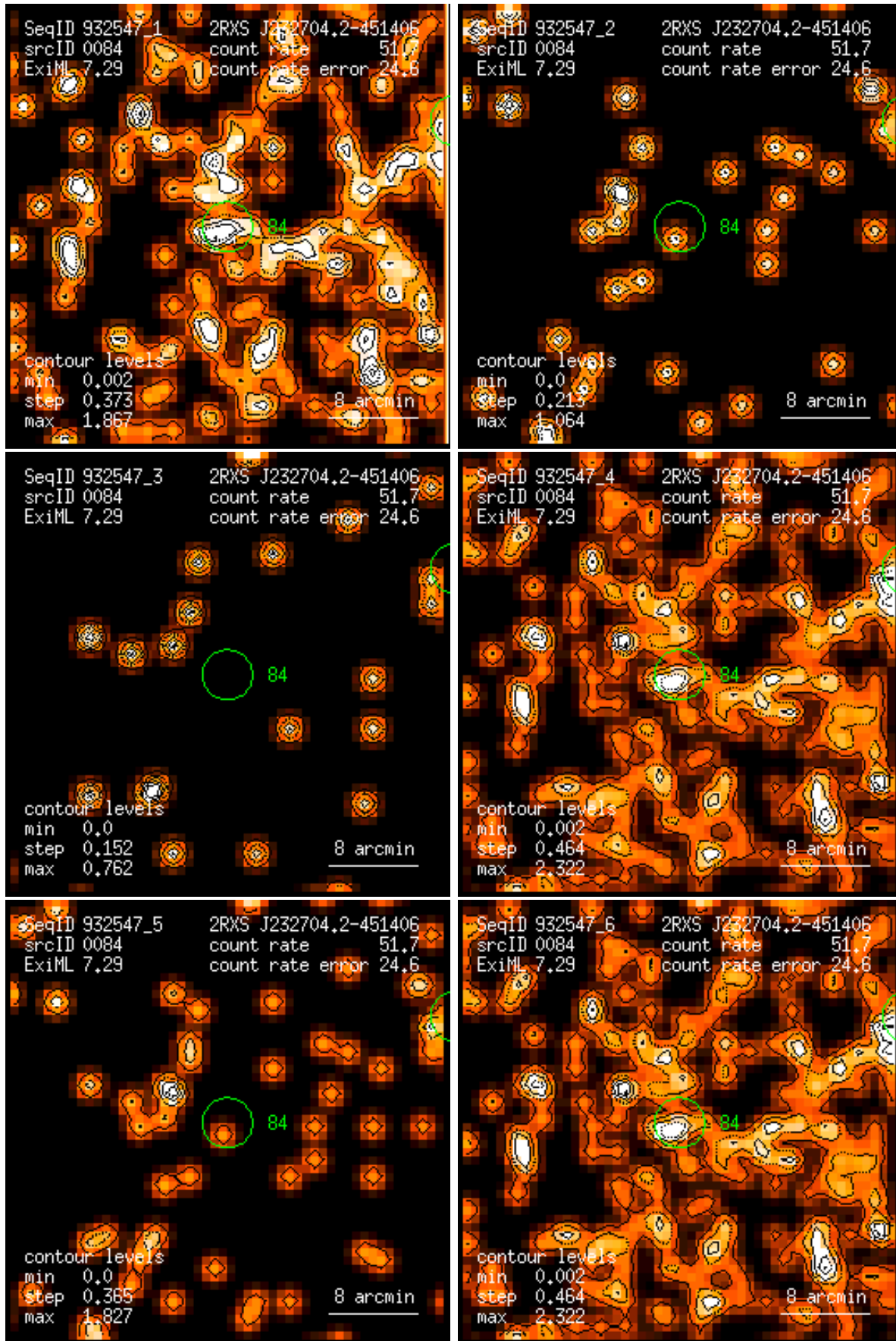
Figure 84: RASS 932547: detection 0084: band rate images, Gaussian filter: (1) PSPC channels 11 – 41, (2) 52 – 90, (3) 91 – 201, (4) 11 – 235, (5) 52 – 201, (6) 11 – 201. Broad band rates in counts/ks. Band rate contour levels in counts/ks/arcmin 2 .
