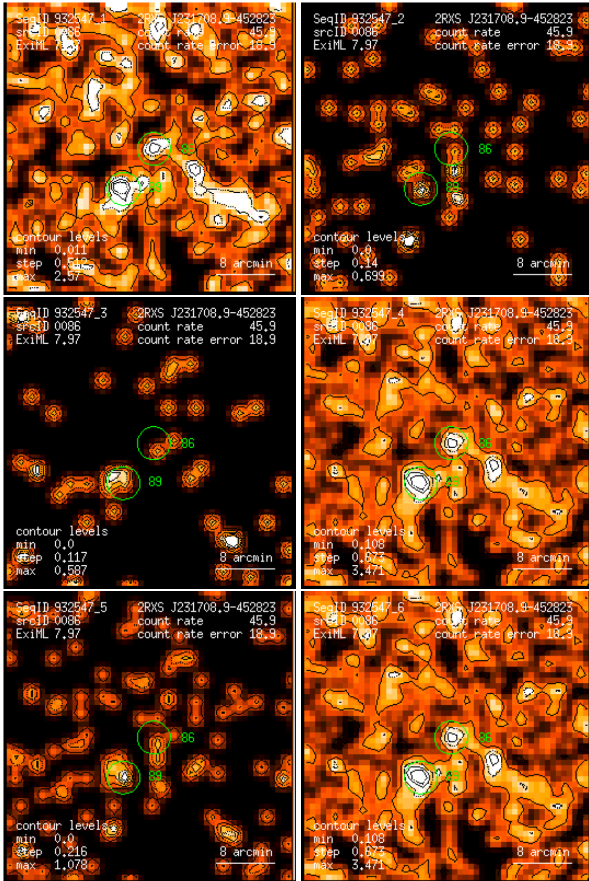
Figure 86: RASS 932547: detection 0086: band rate images, Gaussian filter: (1) PSPC channels 11 – 41, (2) 52 – 90, (3) 91 – 201, (4) 11 – 235, (5) 52 – 201, (6) 11 – 201. Broad band rates in counts/ks. Band rate contour levels in counts/ks/arcmin 2 .
